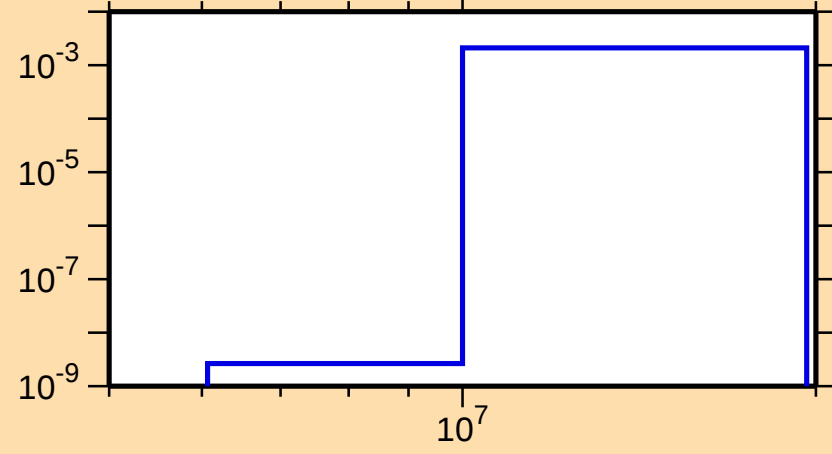
\sigma vs. E for ^{69}\text{Zn}(n,n\alpha)
