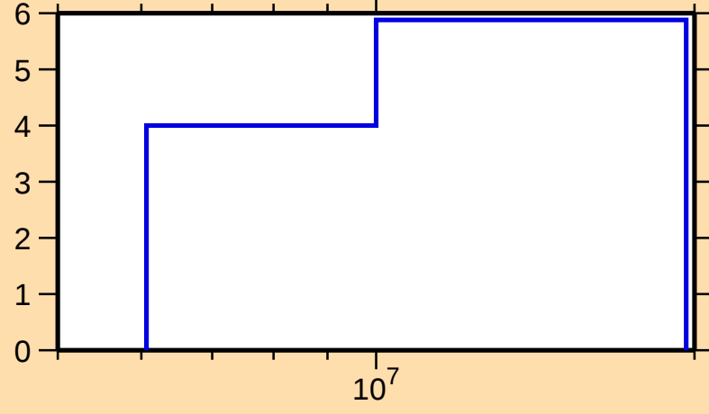
\Delta\sigma/\sigma vs. E for ^{69}\text{Zn}(n,\text{tot.})
