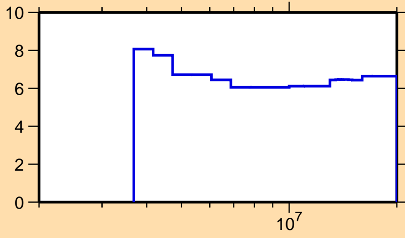
\Delta\sigma/\sigma vs. E for ^{70}\text{Zn}(n,n\text{onl.})
