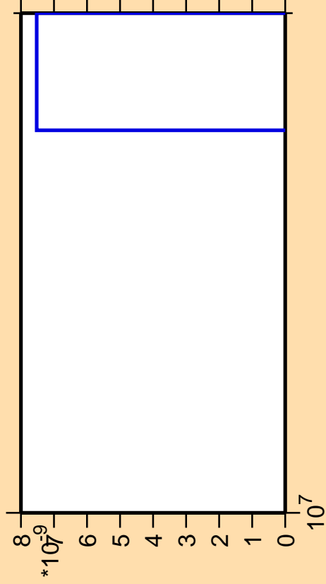
\Delta\sigma/\sigma vs. E for ^{70}\text{Zn}(n,pd)
