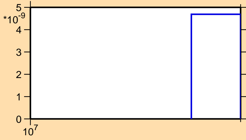
\sigma vs. E for ^{70}\text{Zn}(n,nd)
