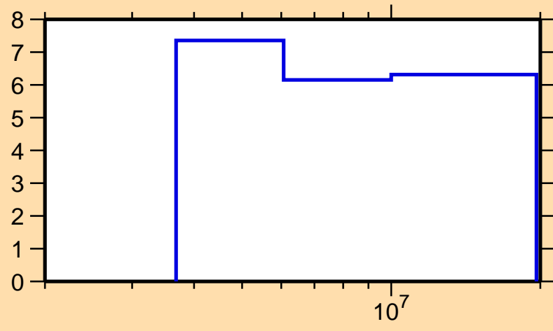
\Delta\sigma/\sigma vs. E for ^{70}\text{Zn}(n,n\text{onel.})
