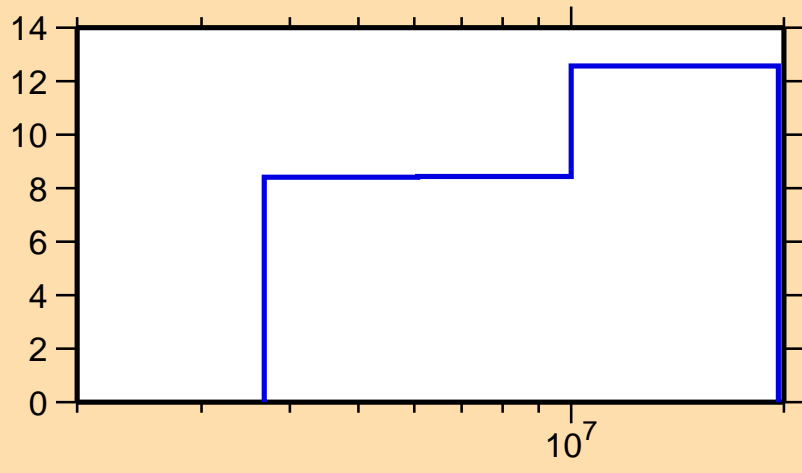
\Delta\sigma/\sigma vs. E for ^{70}\text{Zn}(n,el.)
