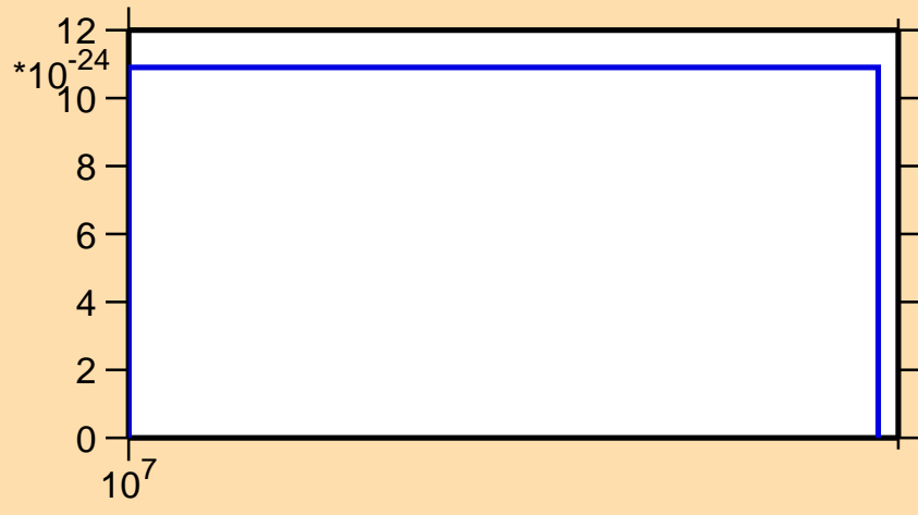
\sigma vs. E for ^{70}\text{Zn}(n,pd)
