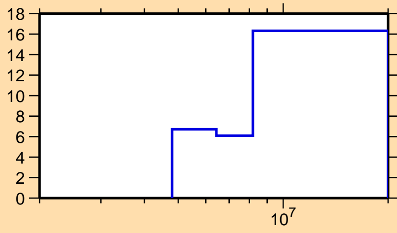
\Delta\sigma/\sigma vs. E for ^{70}\text{Zn}(n,\text{inel.})
