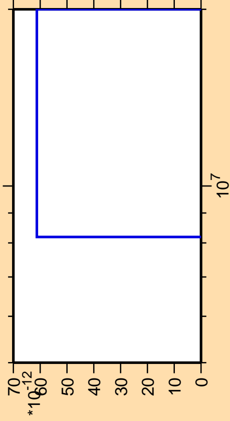
\Delta\sigma/\sigma vs. E for ^{70}\text{Zn}(n,\text{pd})
