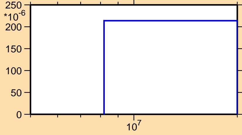
\sigma vs. E for ^{70}\text{Zn}(n,3n)
