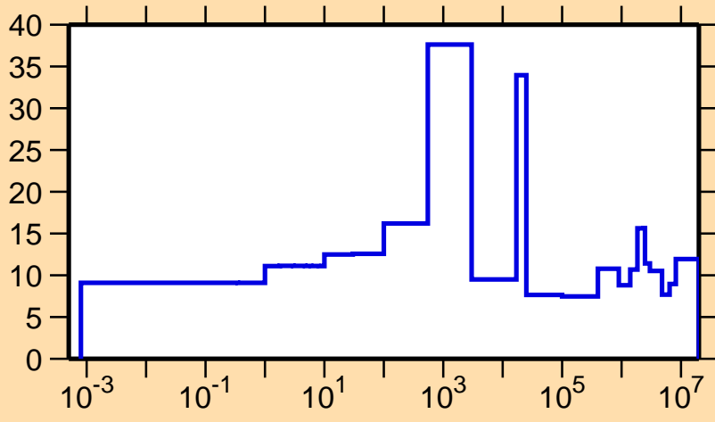
\Delta\sigma/\sigma vs. E for ^{70}\text{Zn}(n,\text{el.})
