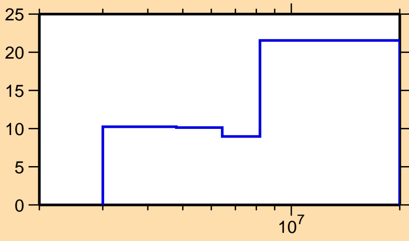
\Delta\sigma/\sigma vs. E for ^{70}\text{Zn}(n,n\text{cont.})
