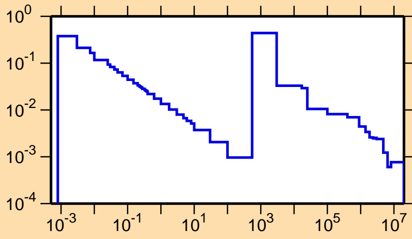
\sigma vs. E for ^{70}\text{Zn}(n,\gamma)
