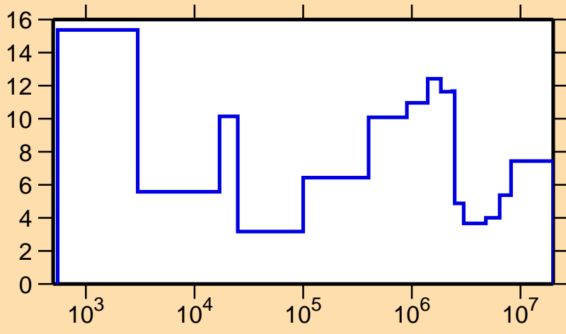
\Delta\sigma/\sigma vs. E for ^{70}\text{Zn}(n,\text{tot.})
