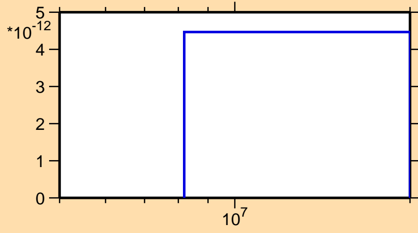
\sigma vs. E for ^{70}\text{Zn}(n,nt)
