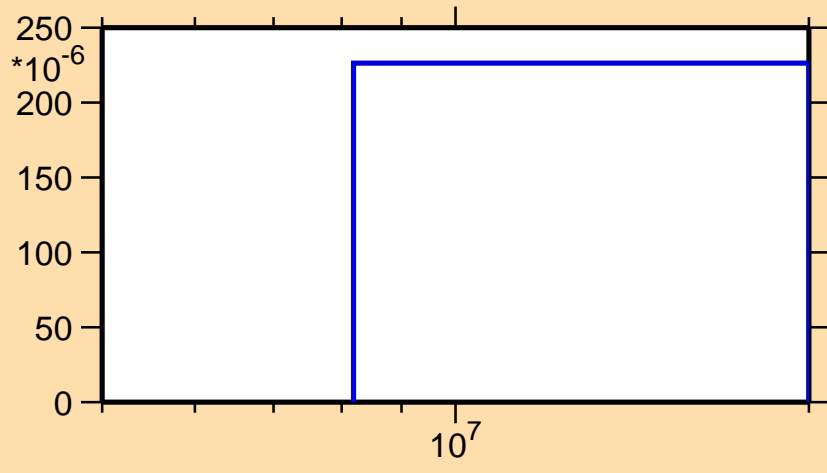
\sigma vs. E for ^{70}\text{Zn}(n,np)
