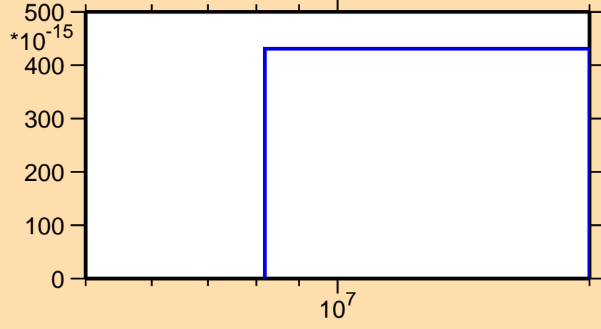
\sigma vs. E for ^{70}\text{Zn}(n,2n\alpha)
