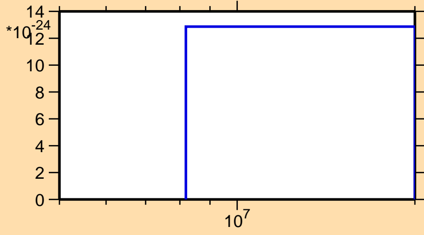
\sigma vs. E for ^{70}\text{Zn}(n,\text{pd})
