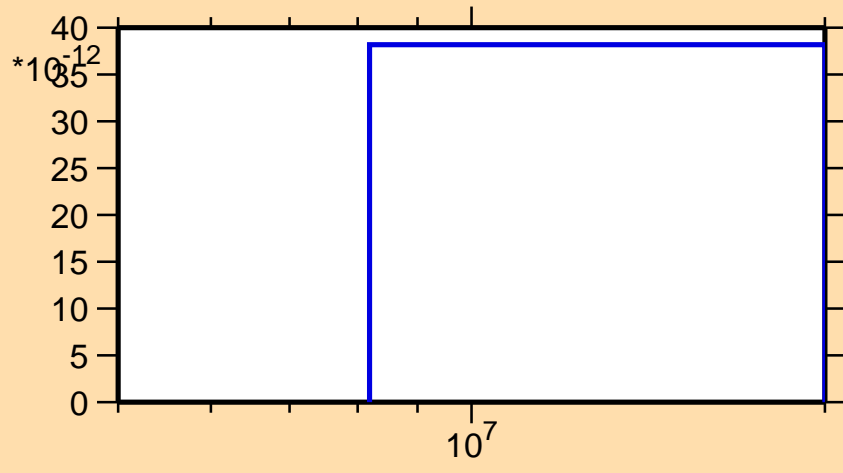
\sigma vs. E for ^{70}\text{Zn}(n,\text{nd})
