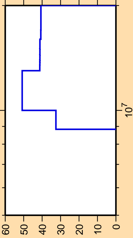
\Delta\sigma/\sigma vs. E for ^{71}\text{Zn}(n,n\alpha)
