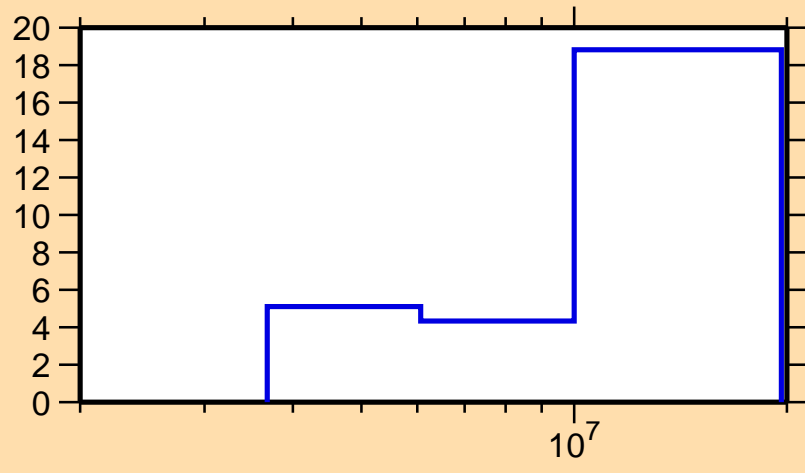
\Delta\sigma/\sigma vs. E for ^{71}\text{Zn}(n,ncont.)
