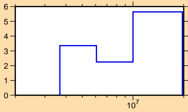
\Delta\sigma/\sigma vs. E for ^{71}\text{Zn}(n,el.)
