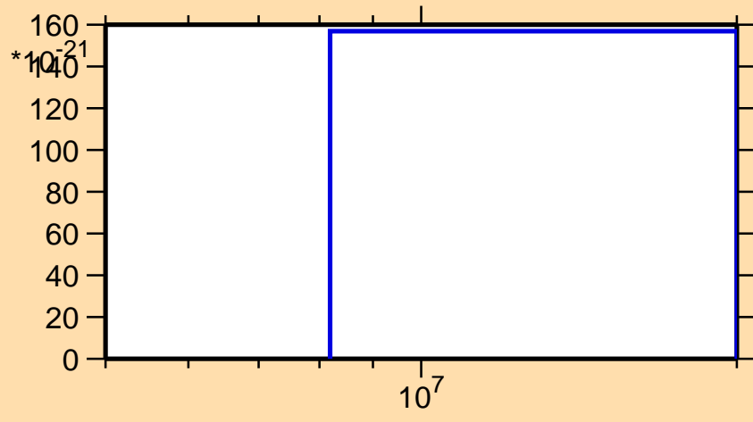
\sigma vs. E for ^{71}\text{Zn} (mt 34)
