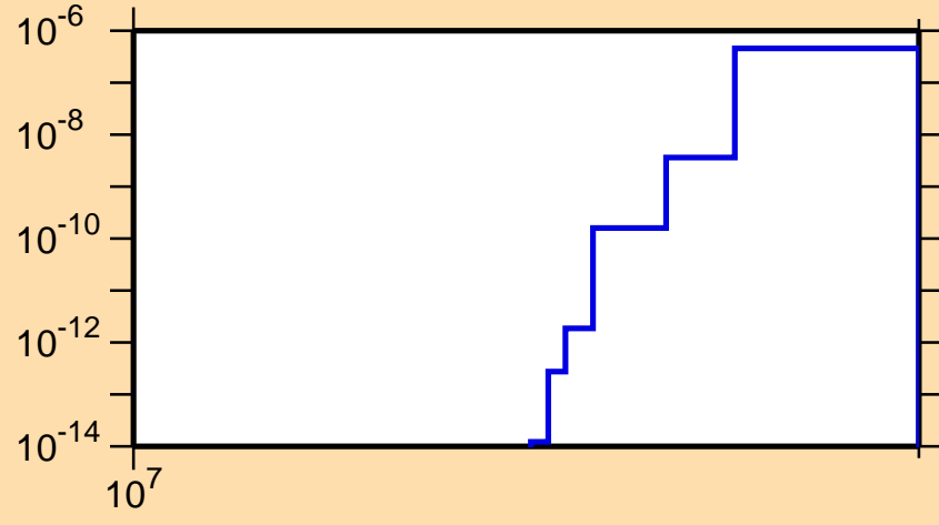
\sigma vs. E for ^{71}\text{Zn}(n,2n\alpha)
