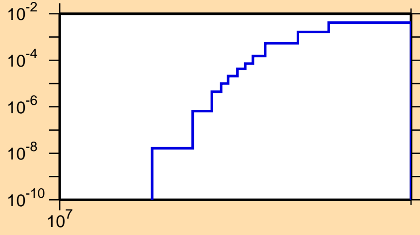
\sigma vs. E for ^{71}\text{Zn}(n,np)
