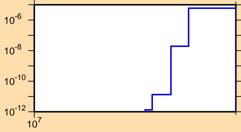
\sigma vs. E for ^{71}\text{Zn}(n,\text{nd})
