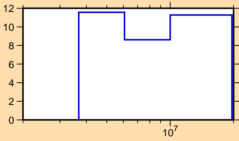
\Delta\sigma/\sigma vs. E for ^{71}\text{Zn}(n,el.)
