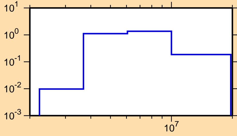
\sigma vs. E for ^{71}\text{Zn}(n,n\text{cont.})
