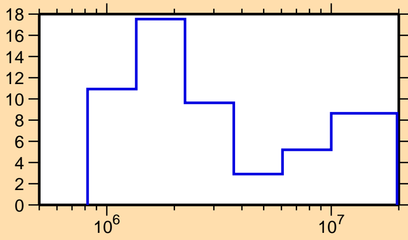
\Delta\sigma/\sigma vs. E for ^{71}\text{Zn}(n,\text{tot.})
