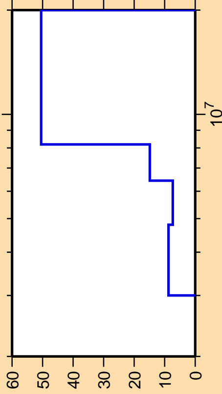
\Delta\sigma/\sigma vs. E for ^{71}\text{Zn}(n,n\text{cont.})
