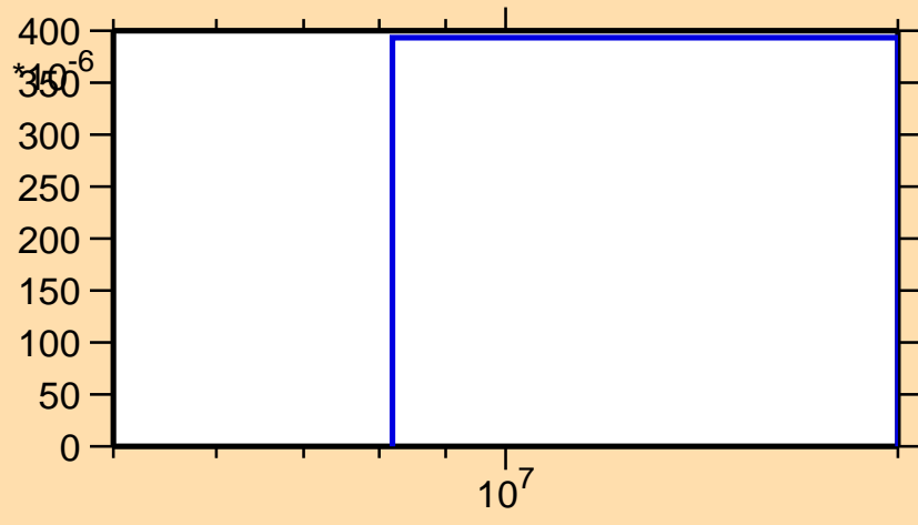
\sigma vs. E for ^{71}\text{Zn}(n,d)
