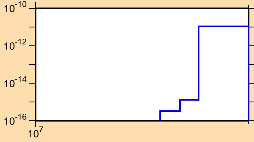
\sigma vs. E for ^{72}\text{Zn}(n,2n\alpha)
