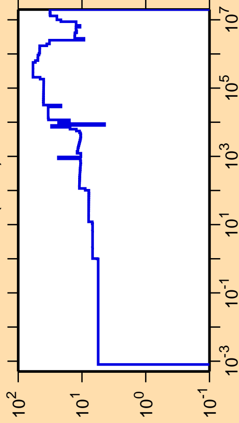
\Delta\sigma/\sigma vs. E for ^{72}\text{Zn}(n,\text{el.})
