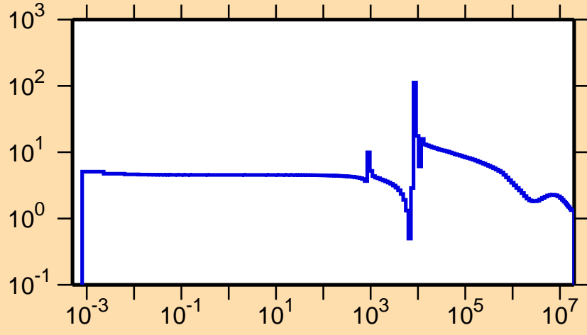
\sigma vs. E for ^{72}\text{Zn}(n,\text{el.})
