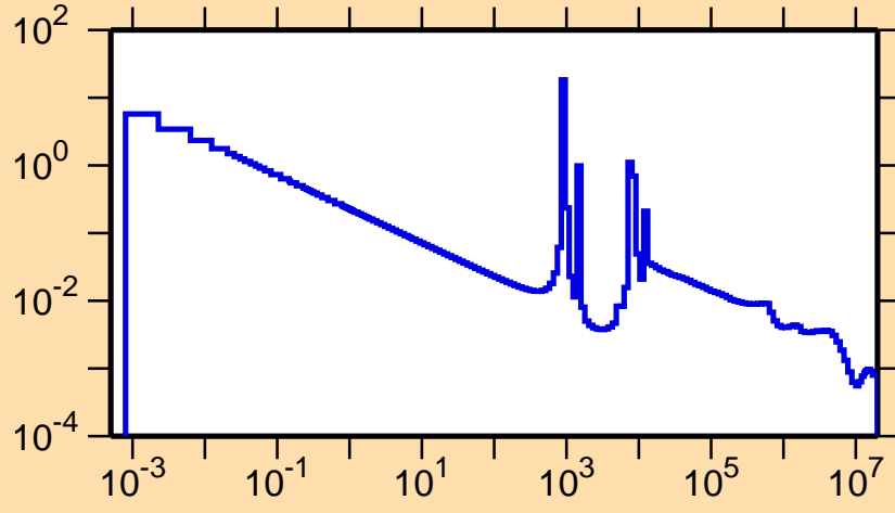
\sigma vs. E for ^{72}\text{Zn}(n,\gamma)
