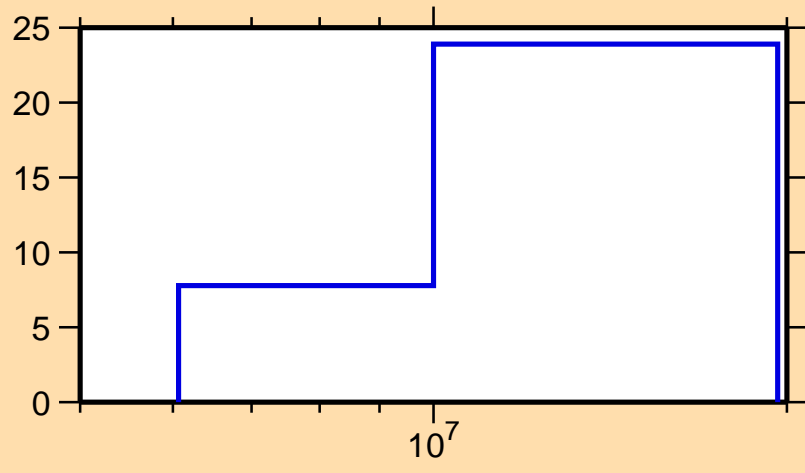
\Delta\sigma/\sigma vs. E for ^{72}\text{Zn}(n,ncont.)
