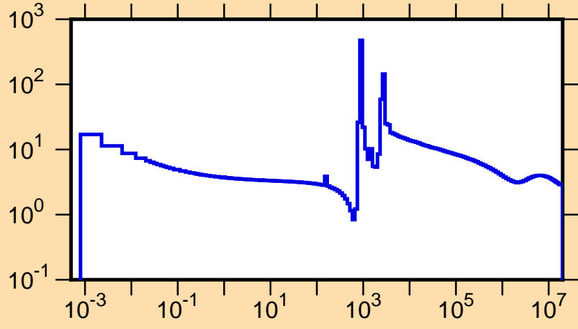
\sigma vs. E for ^{73}\text{Zn}(n,\text{tot.})
