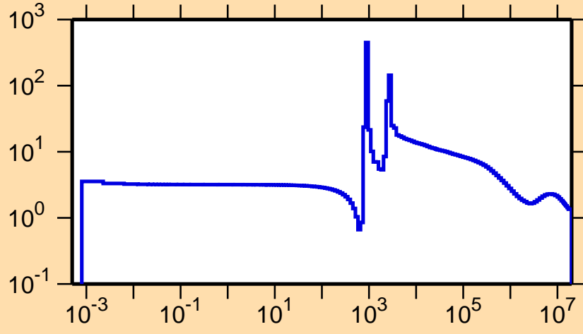
\sigma vs. E for ^{73}\text{Zn}(n,\text{el.})
