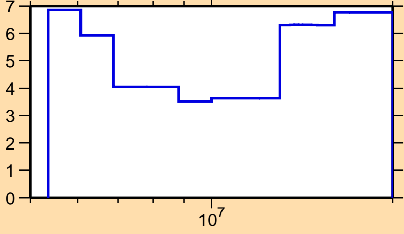
\Delta\sigma/\sigma vs. E for ^{73}\text{Zn}(n,\text{nonel.})
