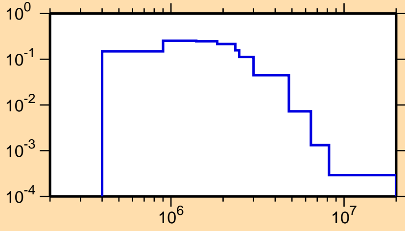
\sigma vs. E for ^{73}\text{Zn}(n,n_4)
