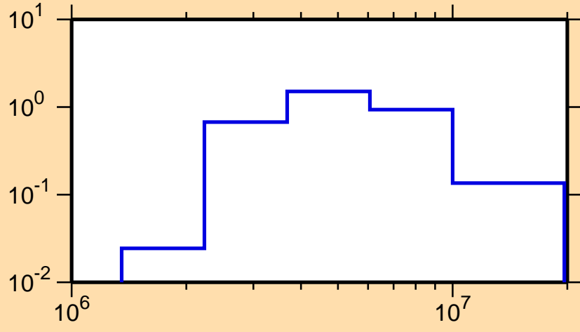
\sigma vs. E for ^{73}\text{Zn}(n,n\text{cont.})
