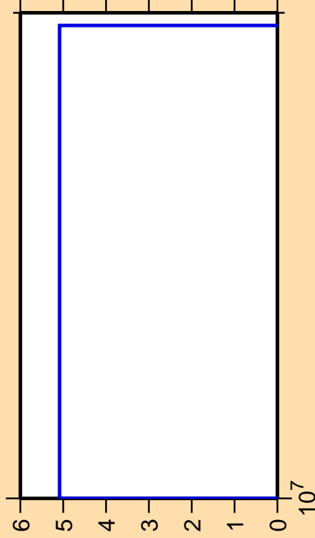
\Delta\sigma/\sigma vs. E for ^{73}\text{Zn}(n,2np)
