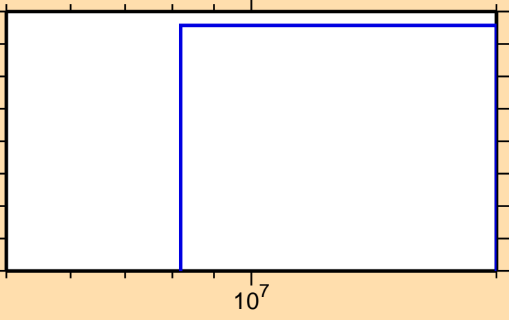
\sigma vs. E for ^{73}\text{Zn}(n,3n)
