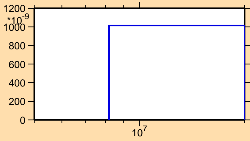
\sigma vs. E for ^{74}\text{Zn}(n,np)
