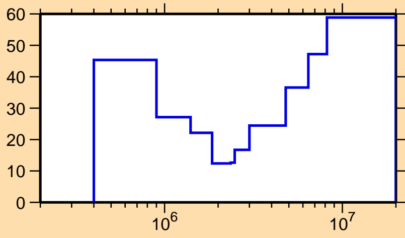
\Delta\sigma/\sigma vs. E for ^{74}\text{Zn}(n,n_1)
