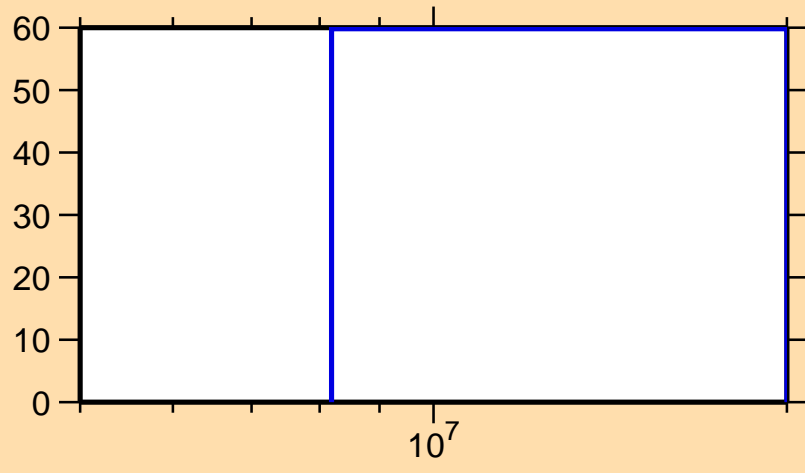
\Delta\sigma/\sigma vs. E for ^{74}\text{Zn}(n,ncont.)
