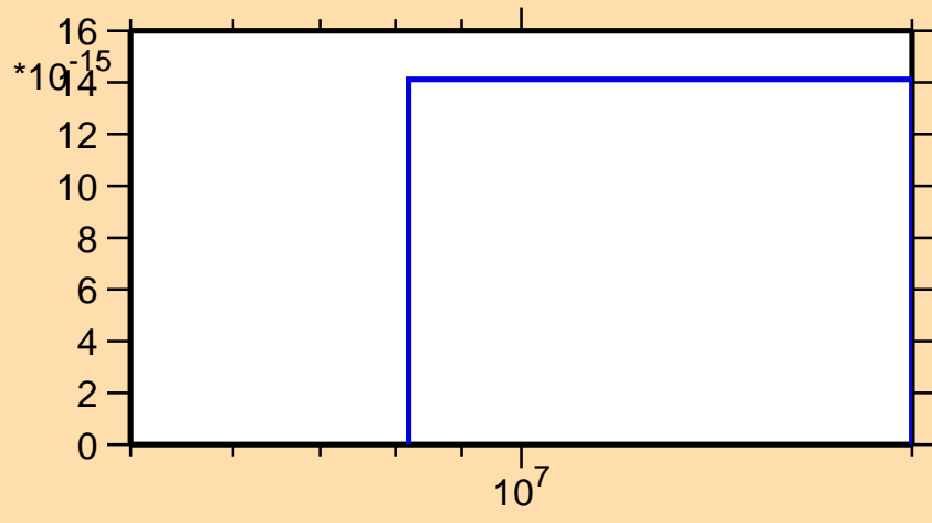
\sigma vs. E for ^{74}\text{Zn}(n,nt)
