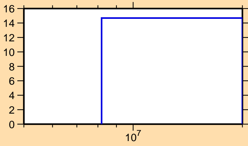
\Delta\sigma/\sigma vs. E for ^{74}\text{Zn}(n,el.)
