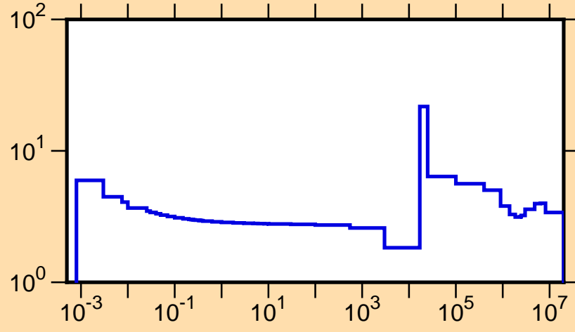
\sigma vs. E for ^{74}\text{Zn}(n,\text{tot.})
