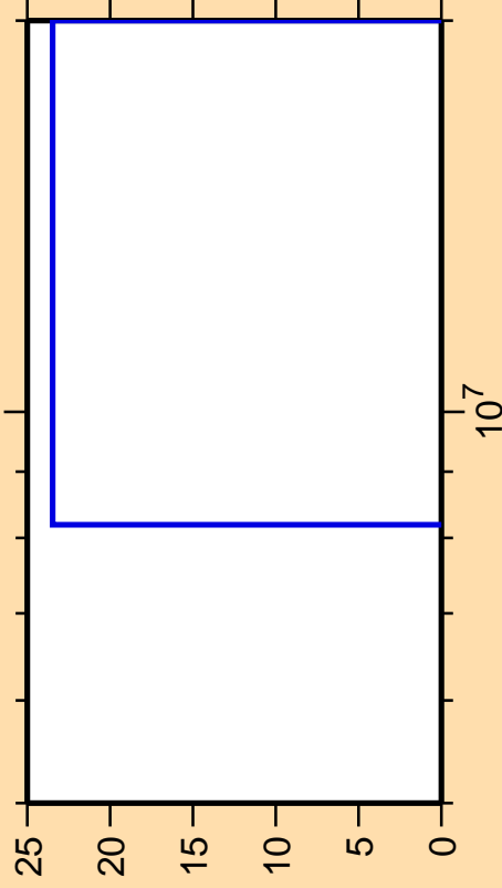
\Delta\sigma/\sigma vs. E for ^{74}\text{Zn}(n,2n)
