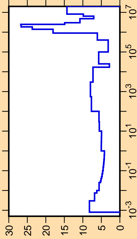
\Delta\sigma/\sigma vs. E for ^{74}\text{Zn}(n,\text{tot.})
