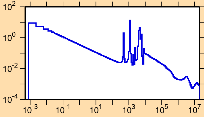
\sigma vs. E for ^{75}\text{Zn}(n,\gamma)
