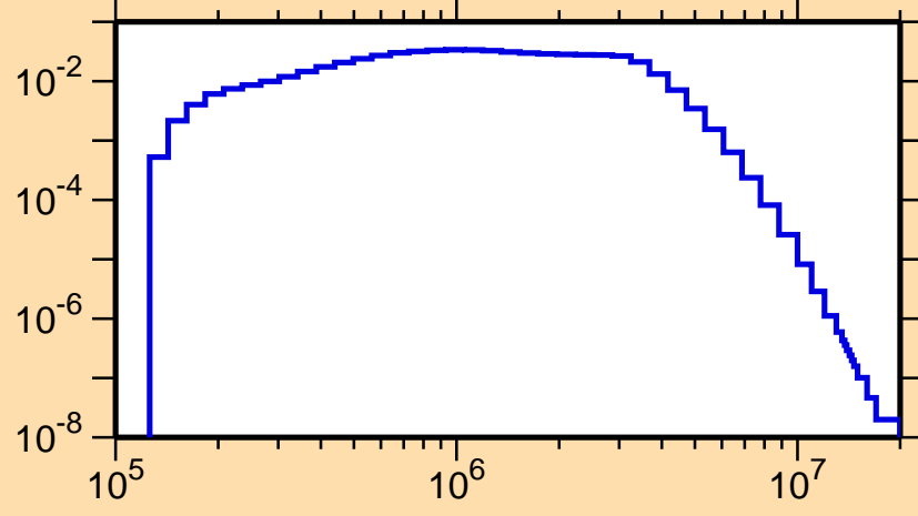
\sigma vs. E for ^{75}\text{Zn}(n,n_1)
