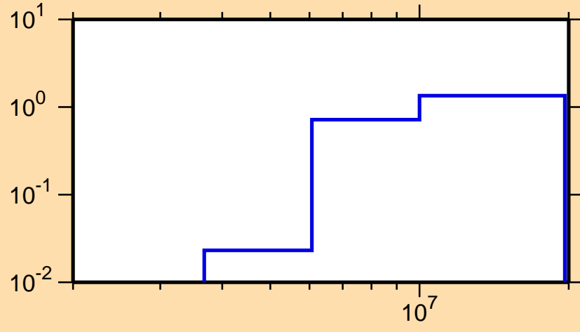
\sigma vs. E for ^{75}\text{Zn}(n,2n)
