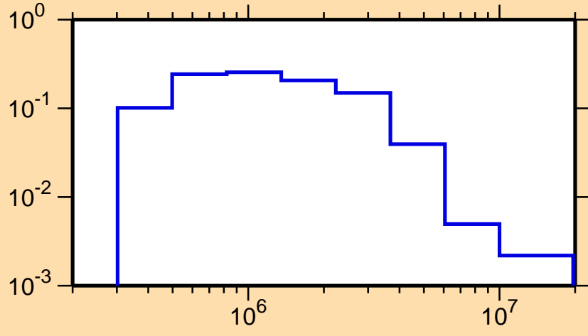
\sigma vs. E for ^{75}\text{Zn}(n,n_4)
