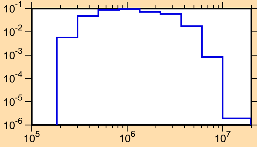
\sigma vs. E for ^{75}\text{Zn}(n,n_3)
