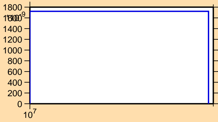
\sigma vs. E for ^{75}\text{Zn}(n,np)
