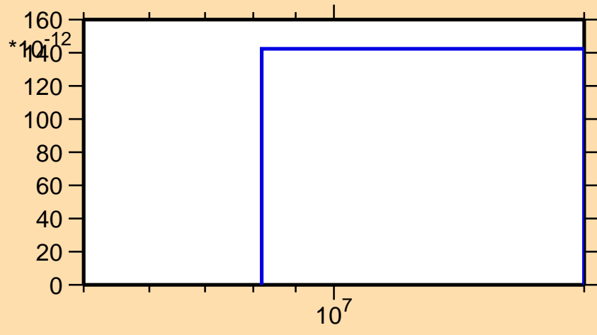
\sigma vs. E for ^{75}\text{Zn}(n,\text{nd})
