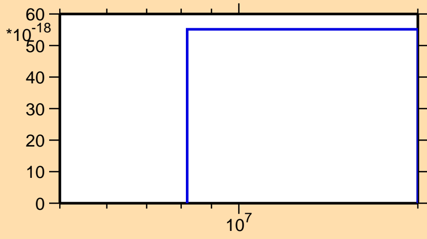
\sigma vs. E for ^{75}\text{Zn}(n,2np)
