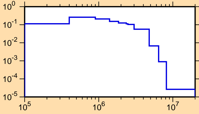
\sigma vs. E for ^{75}\text{Zn}(n,n_2)
