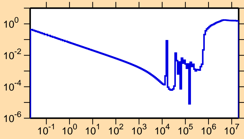
\sigma vs. E for ^{76}\text{Zn}(n,\text{nonel.})
