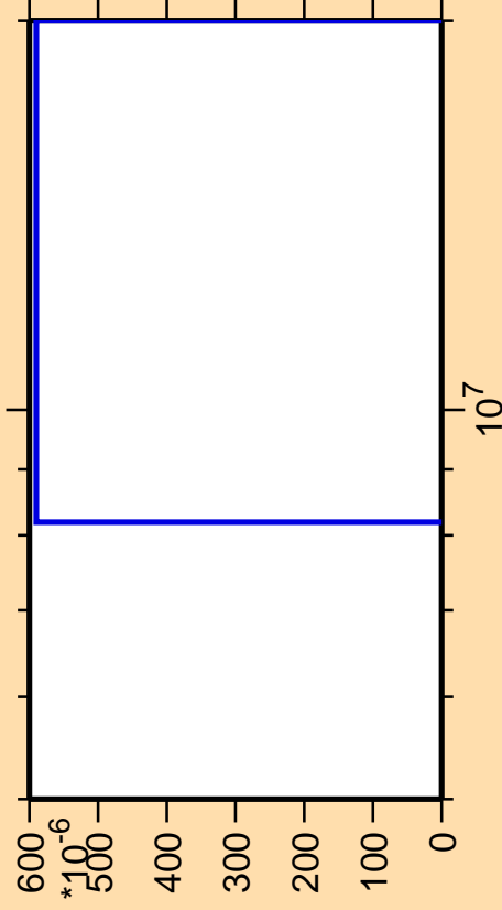
\Delta\sigma/\sigma vs. E for ^{76}\text{Zn}(n,\text{nd})
