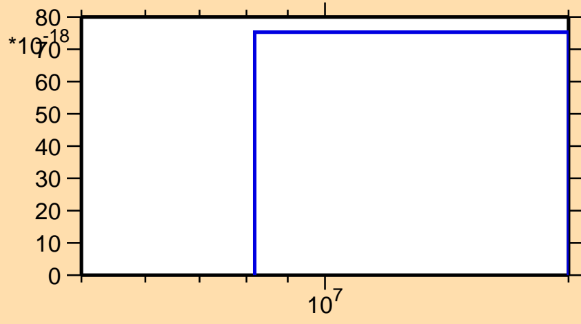
\sigma vs. E for ^{76}\text{Zn}(n,\text{nd})
