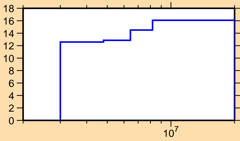
\Delta\sigma/\sigma vs. E for ^{76}\text{Zn}(n,n\text{onel.})
