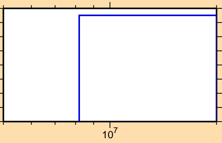
\sigma vs. E for ^{76}\text{Zn}(n,n\alpha)
