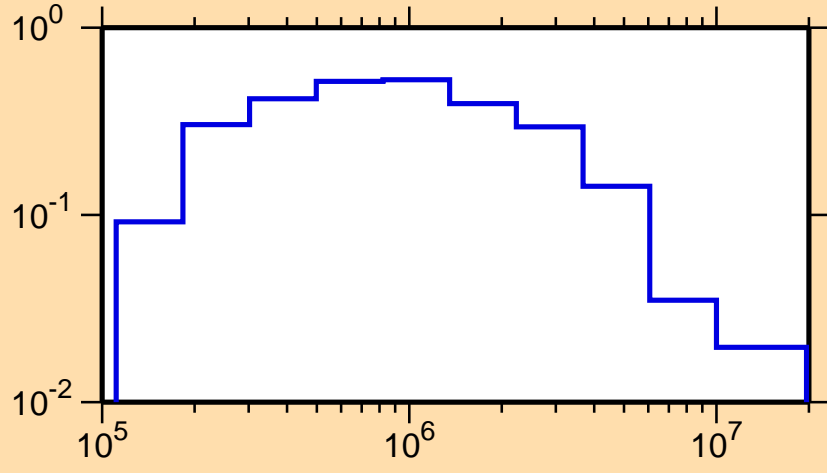
\sigma vs. E for ^{77}\text{Zn}(n,n_1)
