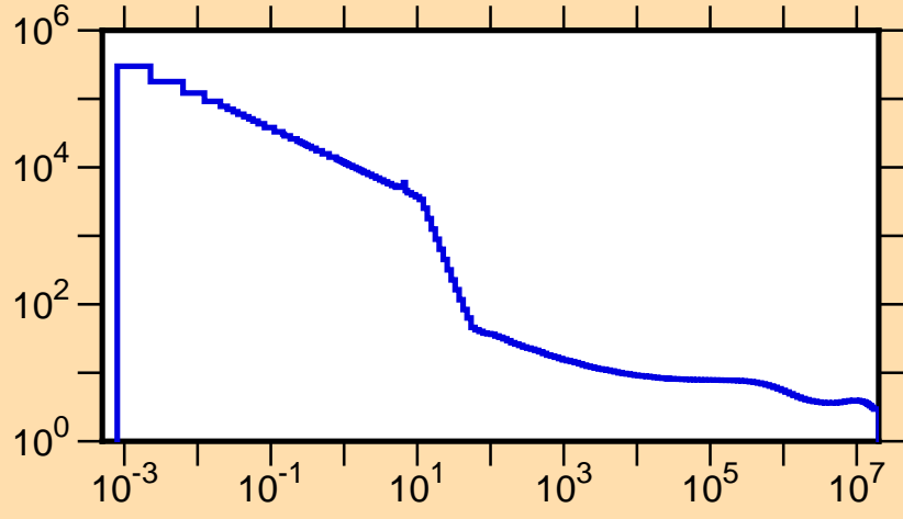
\sigma vs. E for ^{80}\text{Zr}(n,\text{tot.})
