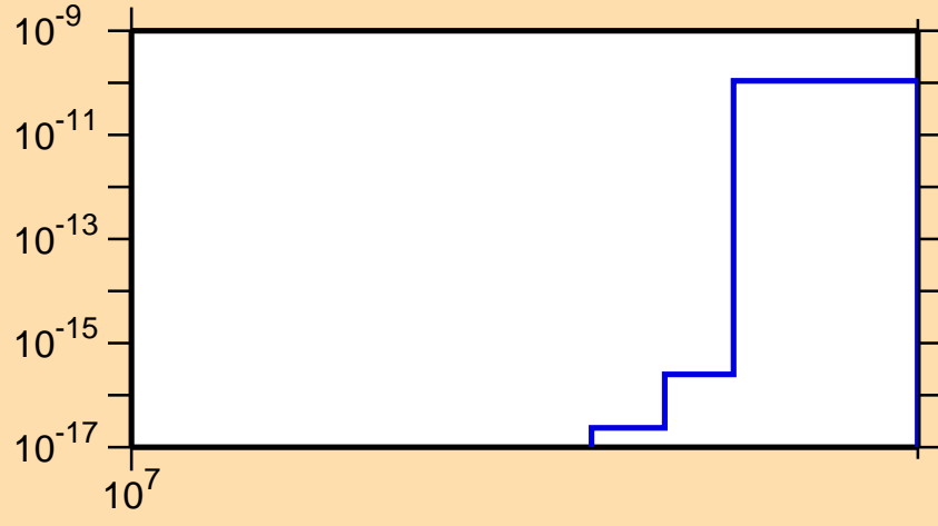
\sigma vs. E for ^{80}\text{Zr}(n,nd)
