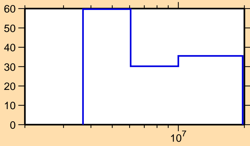
\Delta\sigma/\sigma vs. E for ^{80}\text{Zr}(n,el.)
