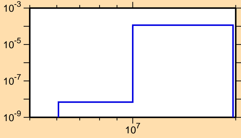
\sigma vs. E for ^{80}\text{Zr}(n,n\alpha)
