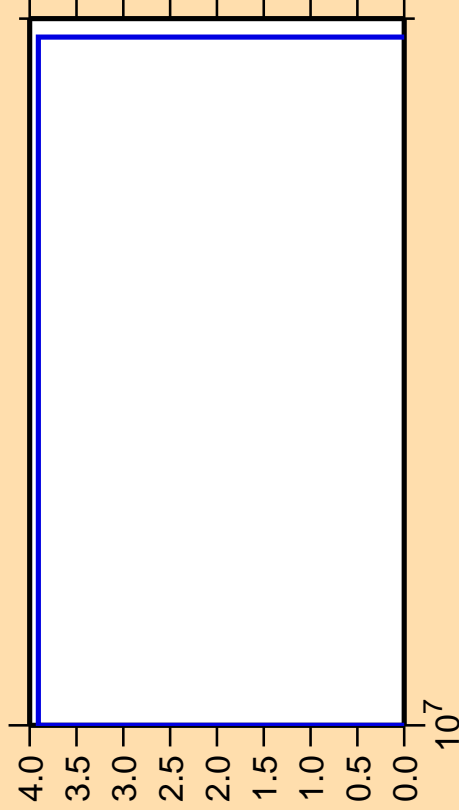
\Delta\sigma/\sigma vs. E for ^{80}\text{Zr}(n,nd)
