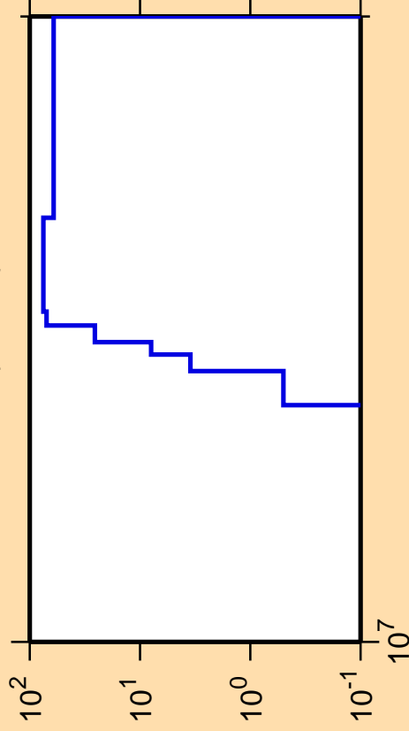
\Delta\sigma/\sigma vs. E for ^{81}\text{Zr} (mt 45)
