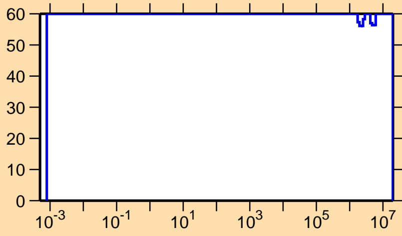
\Delta\sigma/\sigma vs. E for ^{81}\text{Zr}(n,\gamma)
