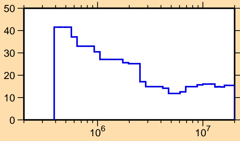
\Delta\sigma/\sigma vs. E for ^{81}\text{Zr}(n,n\text{onel.})
