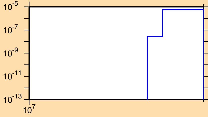
\sigma vs. E for ^{81}\text{Zr}(n,2np)
