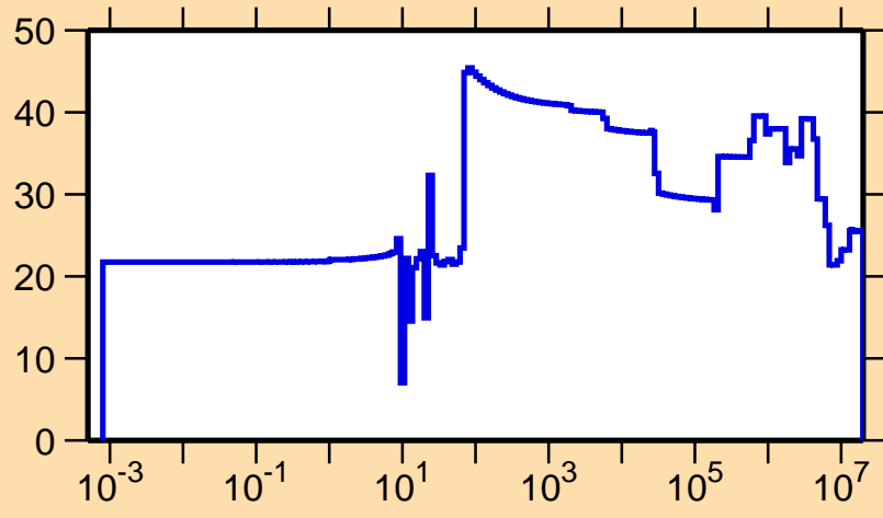
\Delta\sigma/\sigma vs. E for ^{81}\text{Zr}(n,\text{el.})
