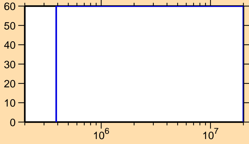
\Delta\sigma/\sigma vs. E for ^{81}\text{Zr}(n,n\text{cont.})
