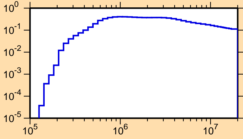
\sigma vs. E for ^{81}\text{Zr}(n,\text{inel.})
