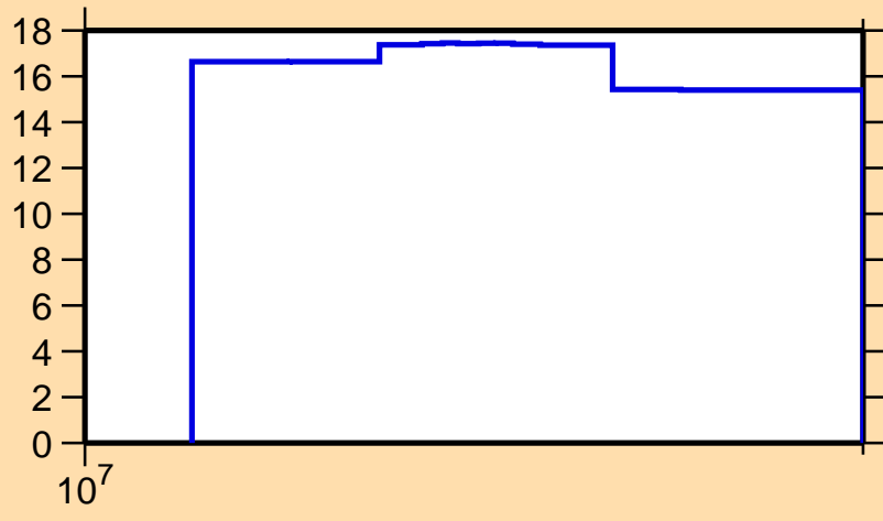
\Delta\sigma/\sigma vs. E for ^{81}\text{Zr}(n,\text{tot.})
