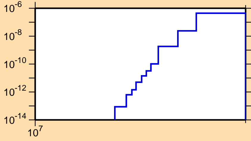
\sigma vs. E for ^{81}\text{Zr}(\text{mt } 34)
