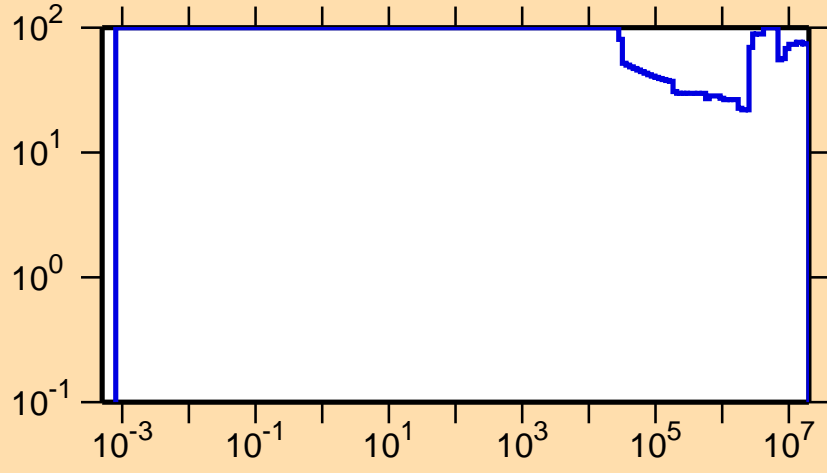
\Delta\sigma/\sigma vs. E for ^{81}\text{Zr}(n,p)
