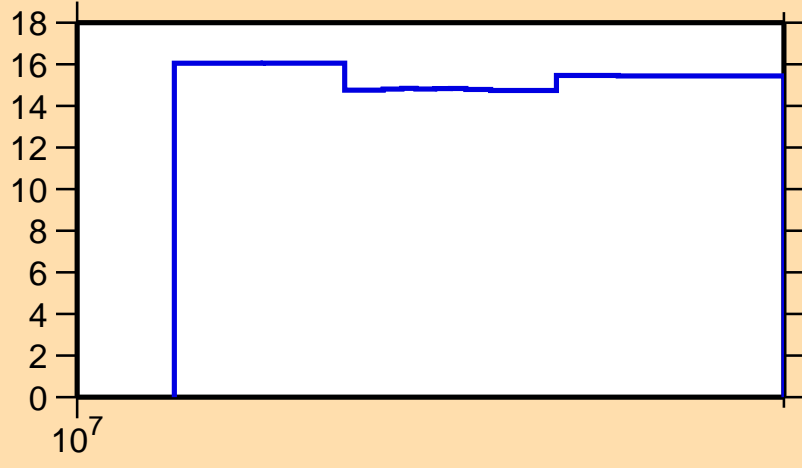
\Delta\sigma/\sigma vs. E for ^{81}\text{Zr}(n,\text{nonel.})
