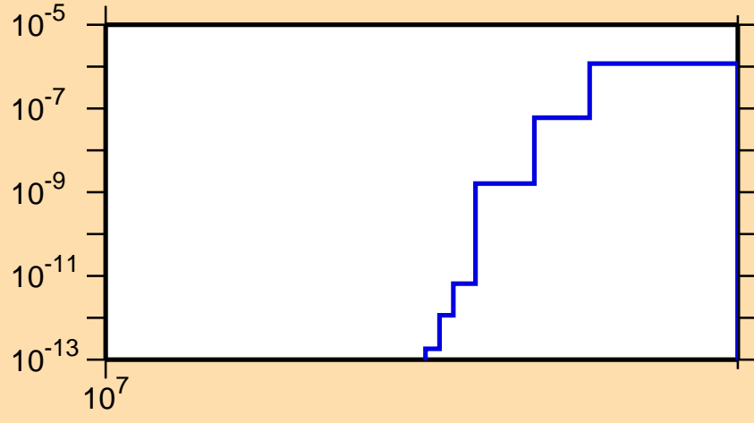
\sigma vs. E for ^{81}\text{Zr}(n,\text{nd})
