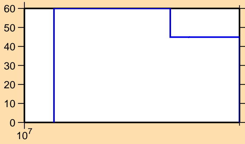
\Delta\sigma/\sigma vs. E for ^{81}\text{Zr}(n,2n)
