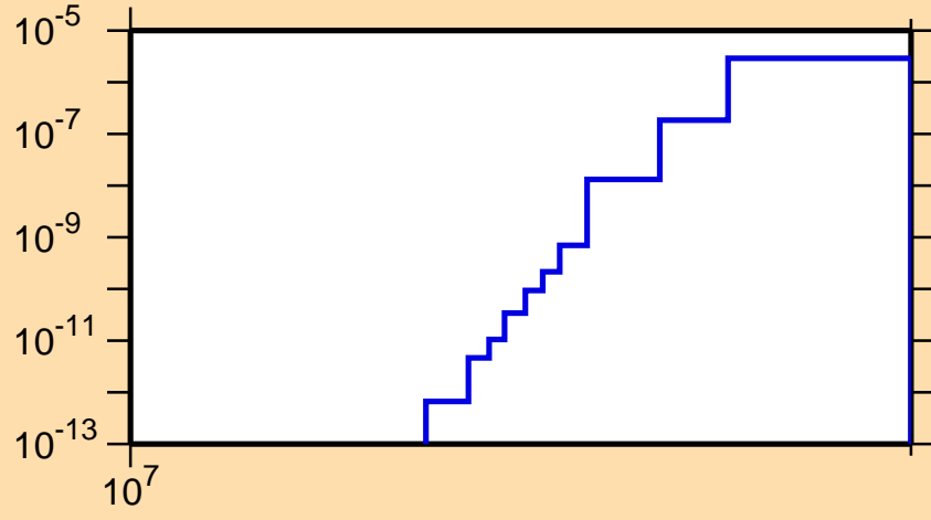
\sigma vs. E for ^{81}\text{Zr} (mt 45)
