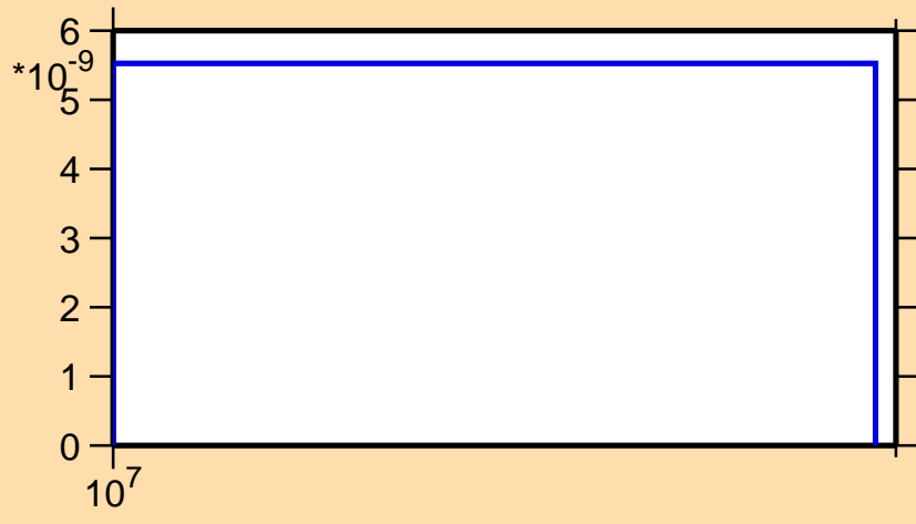
\sigma vs. E for ^{81}\text{Zr} (mt 34)
