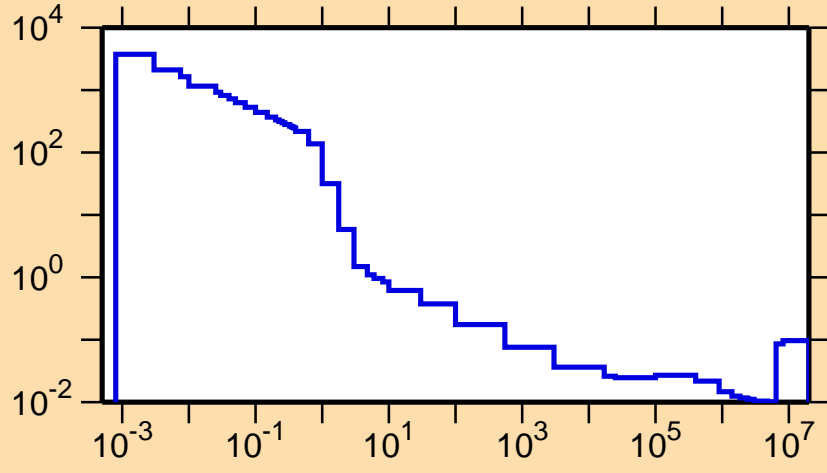
\sigma vs. E for ^{81}\text{Zr}(n,\alpha)
