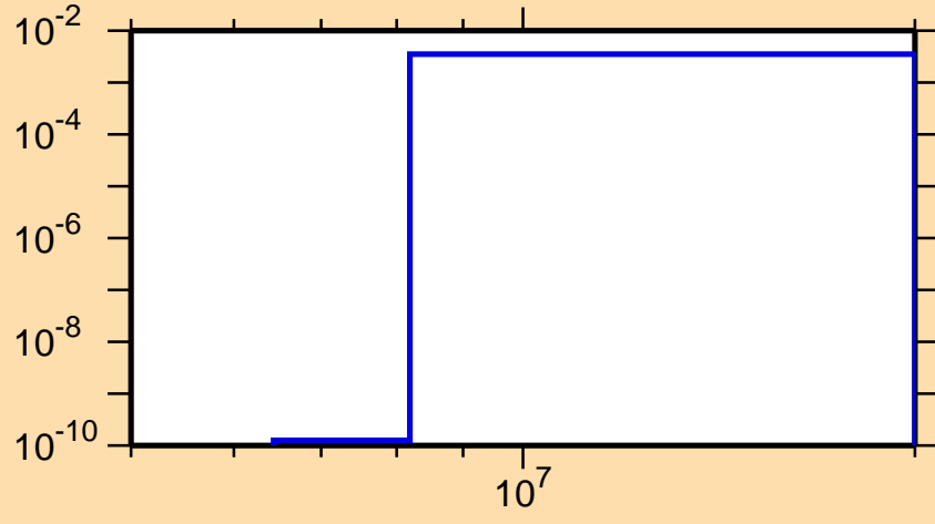
\sigma vs. E for ^{81}\text{Zr}(n,\text{pd})
