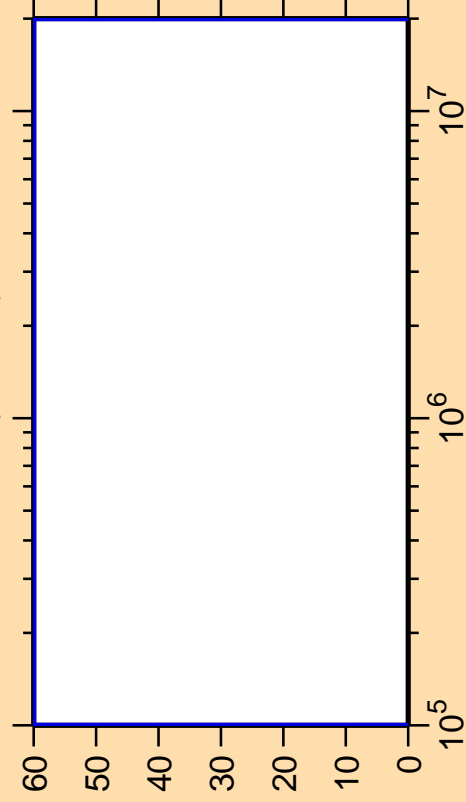
\Delta\sigma/\sigma vs. E for ^{81}\text{Zr}(n,\text{inel.})
