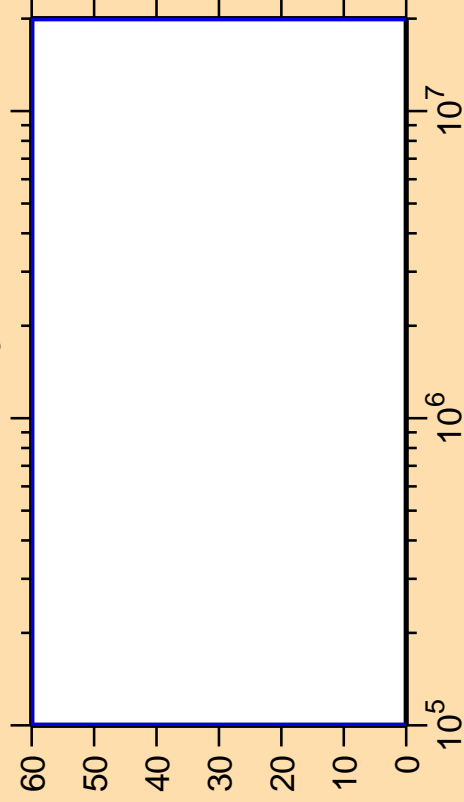
\Delta\sigma/\sigma vs. E for ^{81}\text{Zr}(n,n_3)
