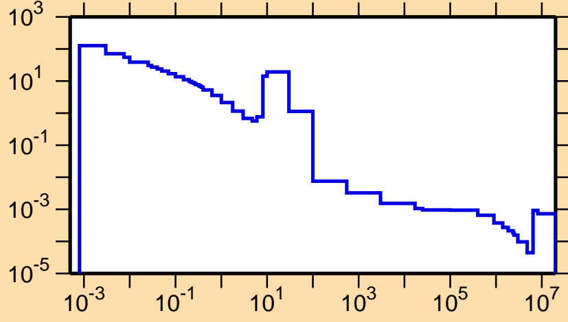
\sigma vs. E for ^{81}\text{Zr}(n,\gamma)
