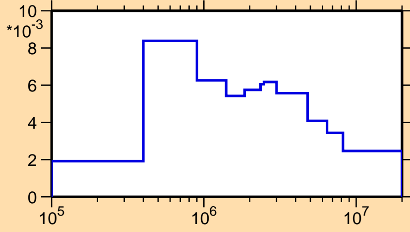
\sigma vs. E for ^{81}\text{Zr}(n,n_2)
