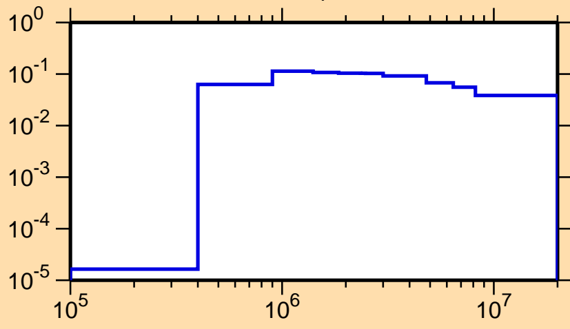
\sigma vs. E for ^{81}\text{Zr}(n,n_4)
