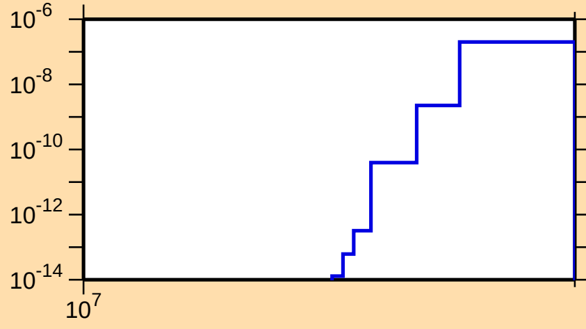
\sigma vs. E for ^{82}\text{Zr}(\text{mt } 45)
