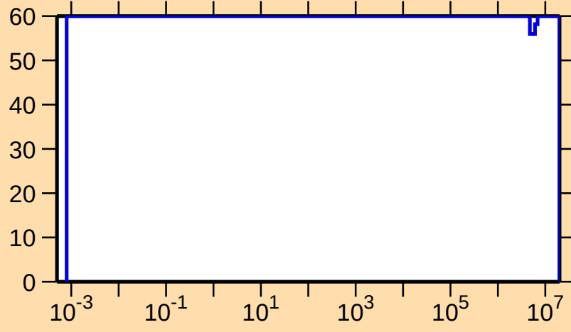
\Delta\sigma/\sigma vs. E for ^{82}\text{Zr}(n,\gamma)
