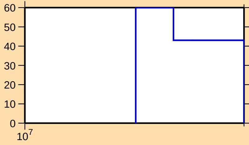
\Delta\sigma/\sigma vs. E for ^{82}\text{Zr}(n,2n)
