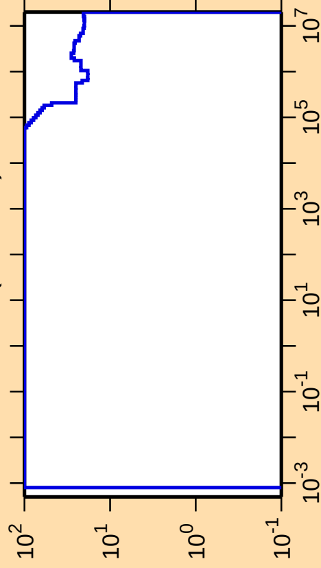
\Delta\sigma/\sigma vs. E for ^{82}\text{Zr}(n,\text{nonel.})
