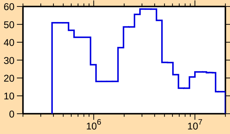
\Delta\sigma/\sigma vs. E for ^{82}\text{Zr}(n,\text{el.})
