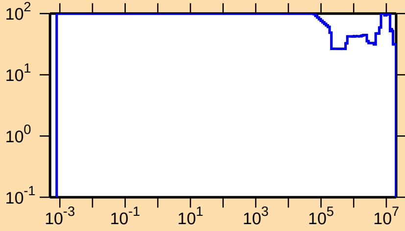
\Delta\sigma/\sigma vs. E for ^{82}\text{Zr}(n,p)
