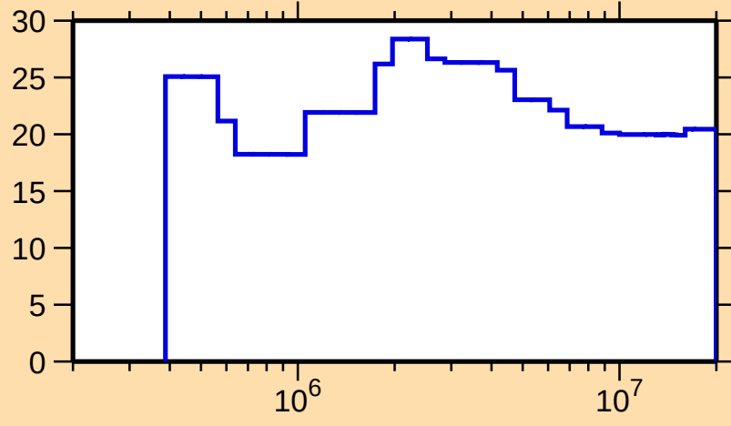
\Delta\sigma/\sigma vs. E for ^{82}\text{Zr}(n,\text{nonel.})
