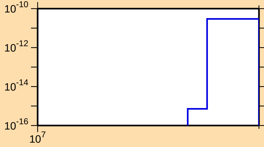
\sigma vs. E for ^{82}\text{Zr}(\text{mt } 34)
