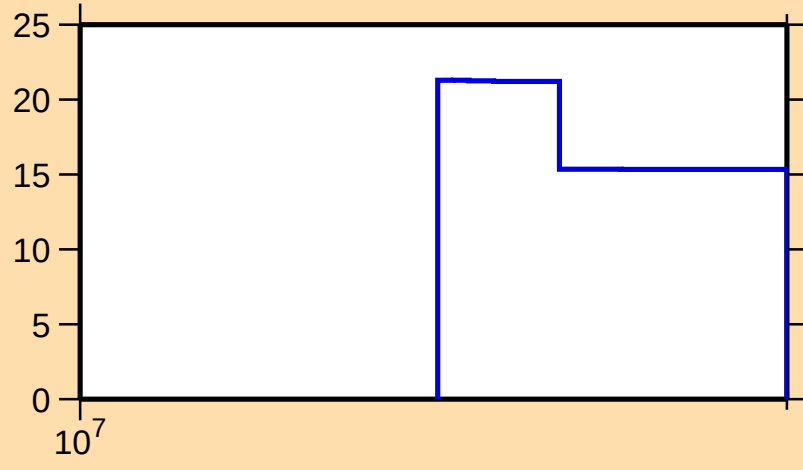
\Delta\sigma/\sigma vs. E for ^{82}\text{Zr}(n,\text{tot.})
