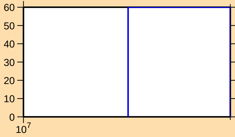
\Delta\sigma/\sigma vs. E for ^{82}\text{Zr}(n,\text{inel.})
