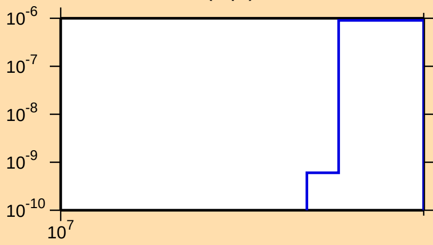
\sigma vs. E for ^{82}\text{Zr}(n,\text{pt})
