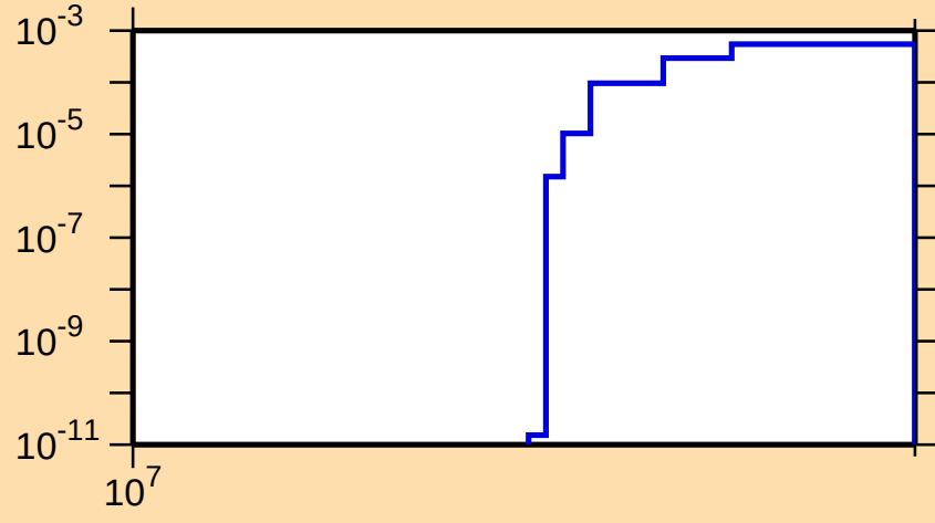
\sigma vs. E for ^{82}\text{Zr}(n,2n)
