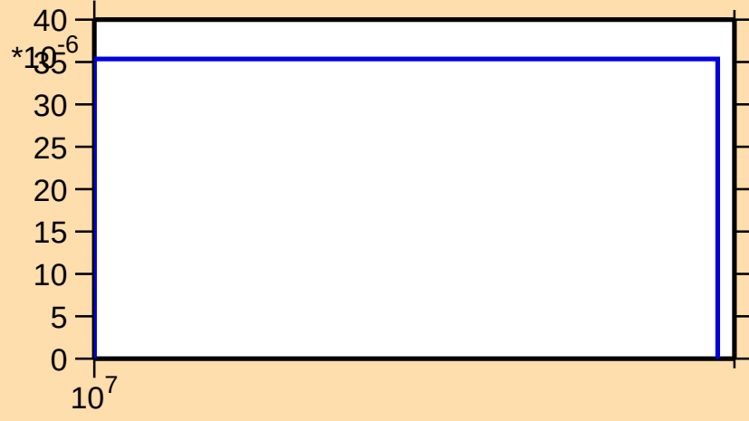
\sigma vs. E for ^{82}\text{Zr}(n,2n)
