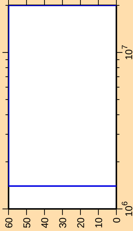
\Delta\sigma/\sigma vs. E for ^{82}\text{Zr}(\text{n},\text{ncont.})
