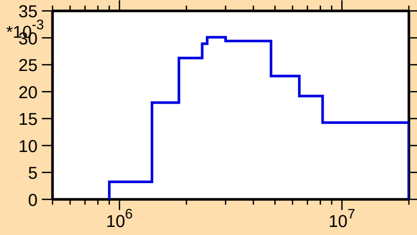
\sigma vs. E for ^{82}\text{Zr}(n,n_2)
