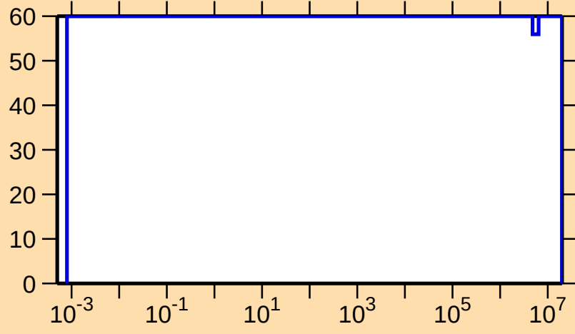
\Delta\sigma/\sigma vs. E for ^{82}\text{Zr}(n,\gamma)
