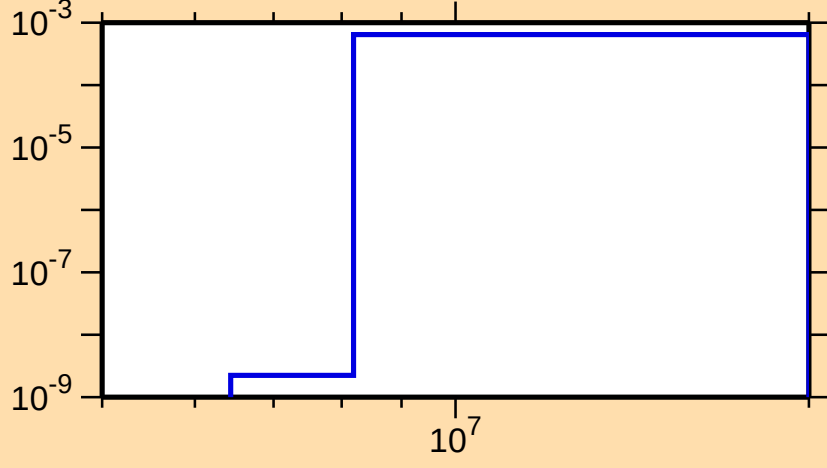
\sigma vs. E for ^{82}\text{Zr}(n,n\alpha)
