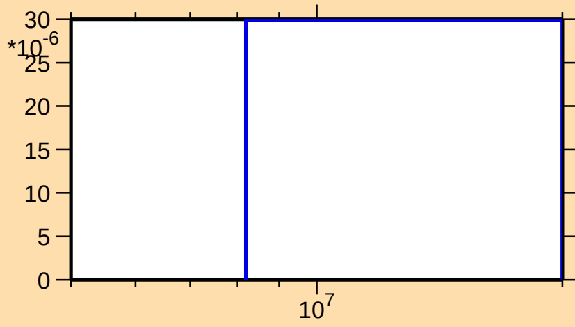
\sigma vs. E for ^{82}\text{Zr}(n,t)
