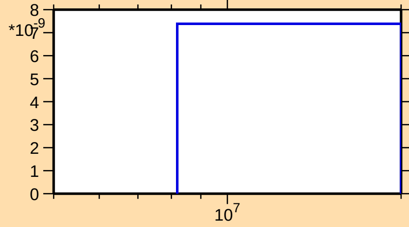
\sigma vs. E for ^{82}\text{Zr}(n,\text{pt})
