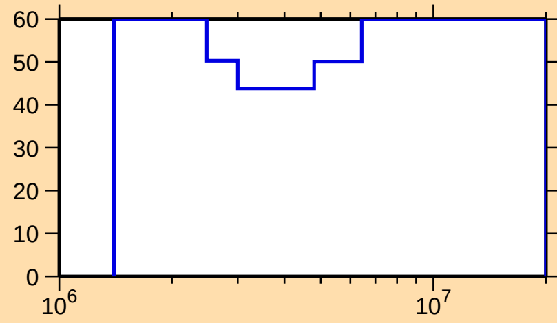
\Delta\sigma/\sigma vs. E for ^{82}\text{Zr}(\text{n},\text{inel.})
