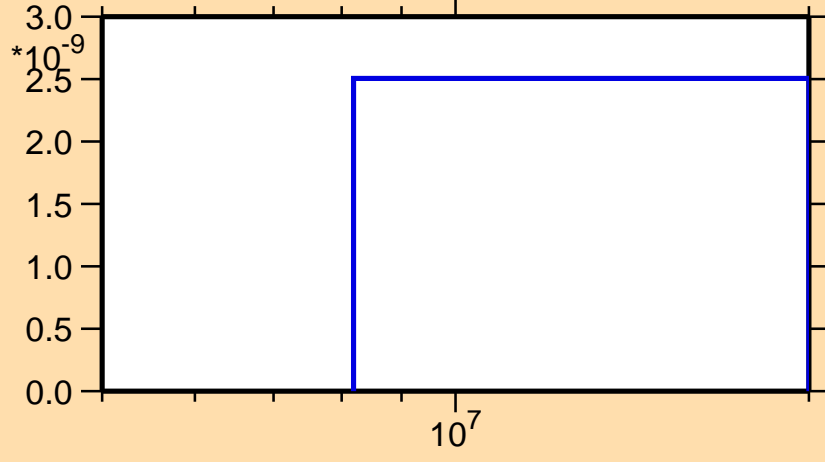
\sigma vs. E for ^{83}\text{Zr}(\text{mt } 34)
