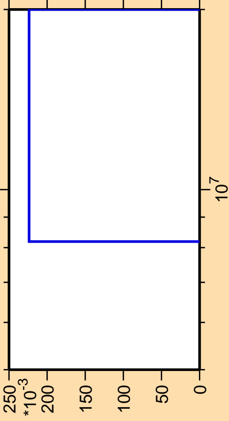
\Delta\sigma/\sigma vs. E for ^{83}\text{Zr}(n,2n\alpha)
