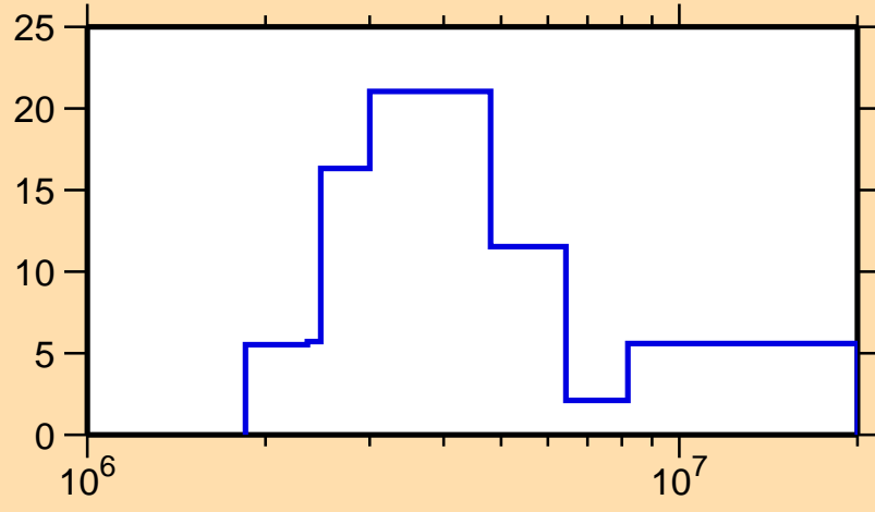
\Delta\sigma/\sigma vs. E for ^{83}\text{Zr}(n, el.)
