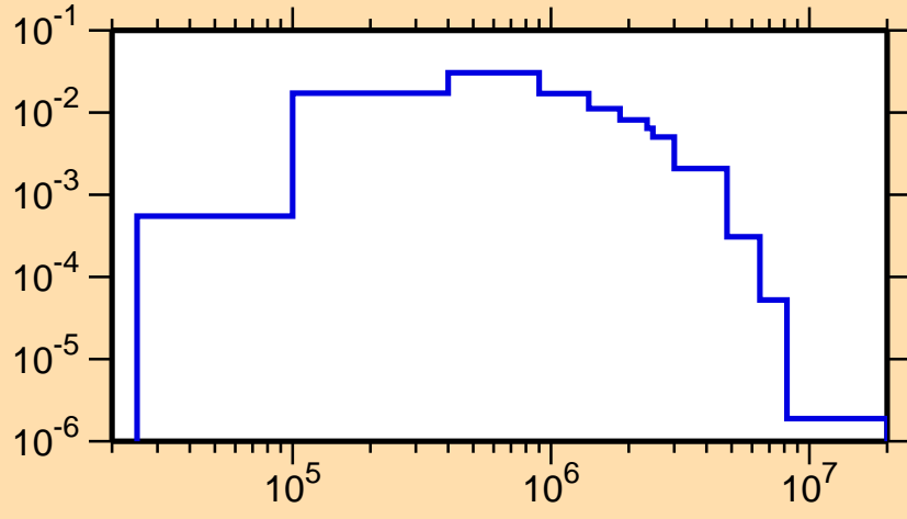
\sigma vs. E for ^{83}\text{Zr}(n,n_1)
