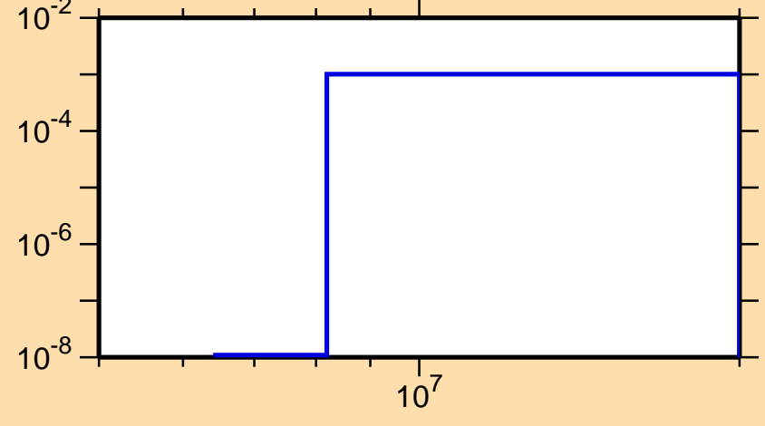
\sigma vs. E for ^{83}\text{Zr}(n,n\alpha)
