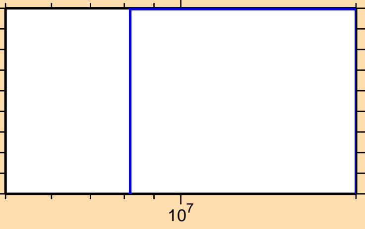
\sigma vs. E for ^{83}\text{Zr}(n,\text{nd})
