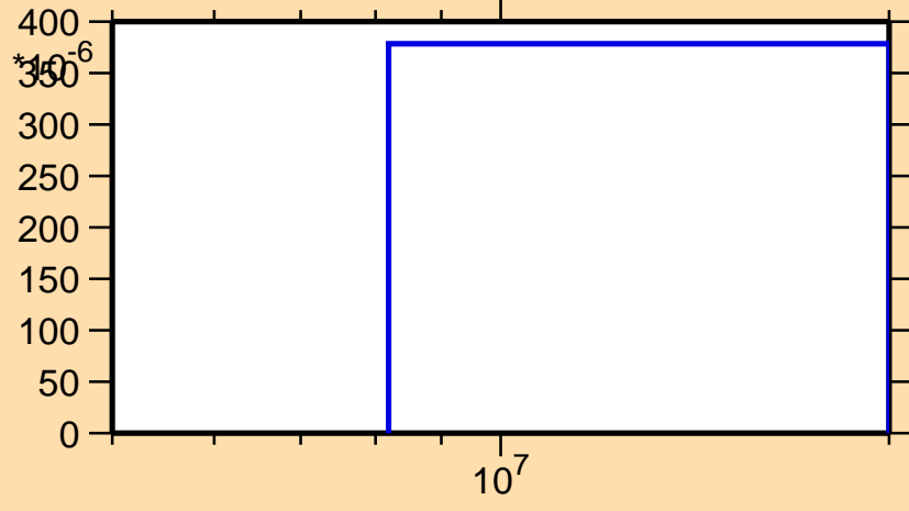
\sigma vs. E for ^{83}\text{Zr}(n,\text{pd})
