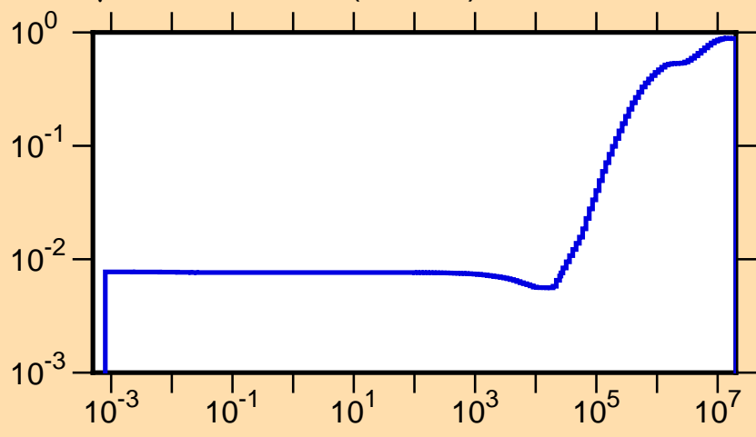
\mu vs. E for ^{87}\text{Zr}(\text{mt251})
