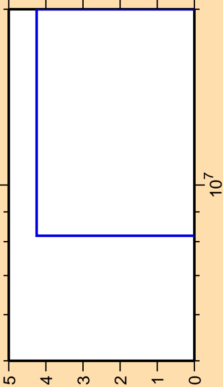
\Delta\sigma/\sigma vs. E for ^{87}\text{Zr}(n,2n\alpha)
