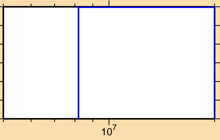
\sigma vs. E for ^{87}\text{Zr}(n,\text{He3})
