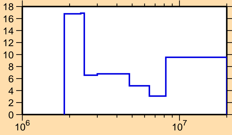
\Delta\sigma/\sigma vs. E for ^{87}\text{Zr}(n,tot.)
