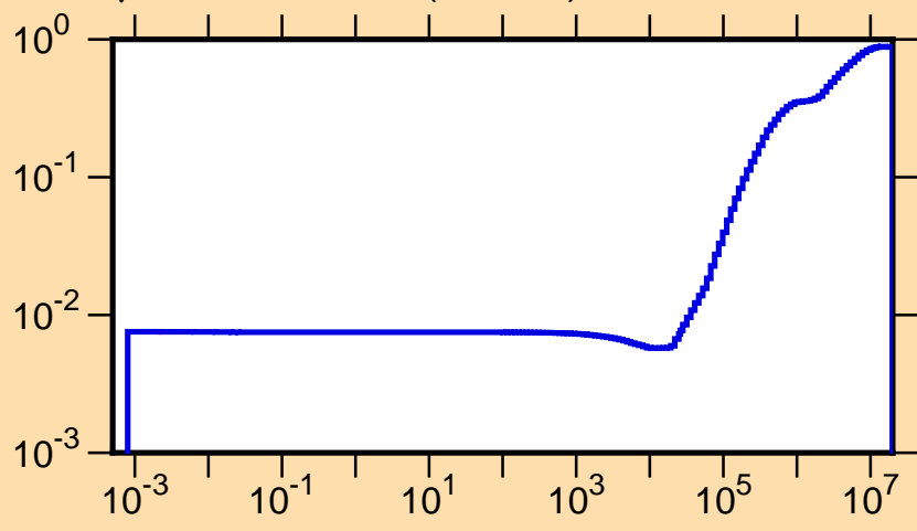
\mu vs. E for ^{89}\text{Zr}(\text{mt251})
