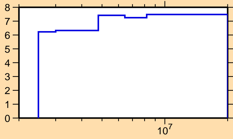
\Delta\sigma/\sigma vs. E for ^{89}\text{Zr}(n,n\text{onel.})
