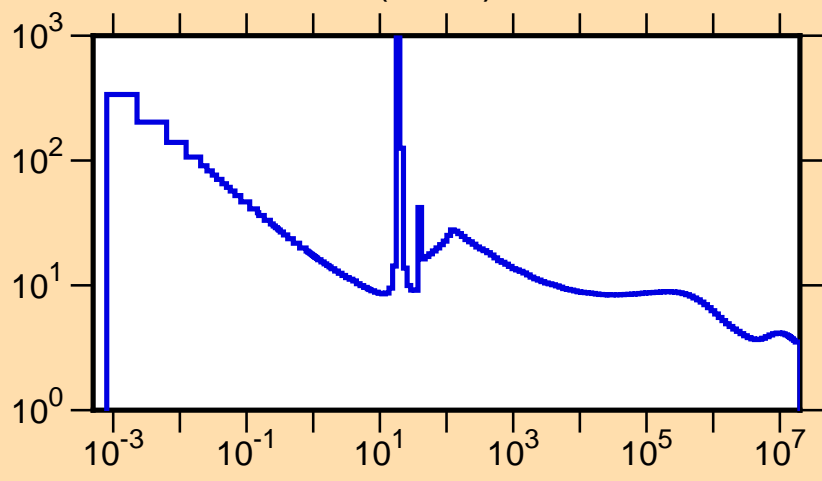
\sigma vs. E for ^{89}\text{Zr}(n,\text{tot.})
