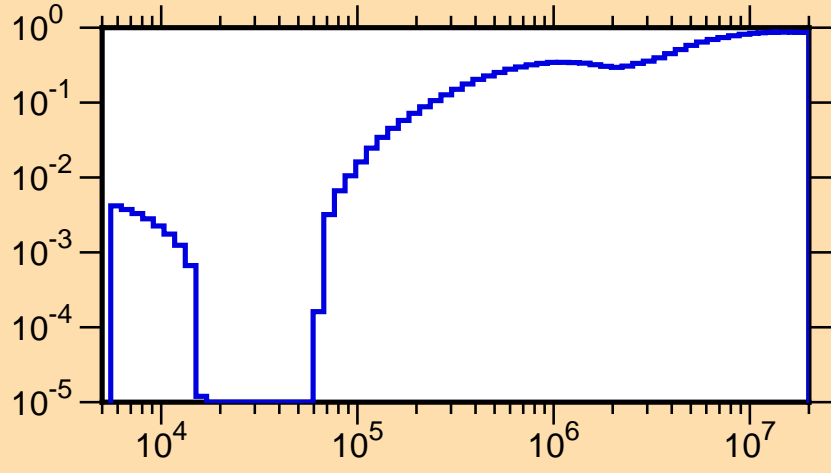
\mu vs. E for ^{90}\text{Zr}(\text{mt251})
