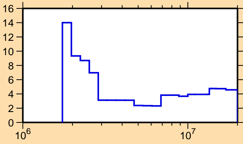
\Delta\sigma/\sigma vs. E for ^{90}\text{Zr}(n,\text{tot.})
