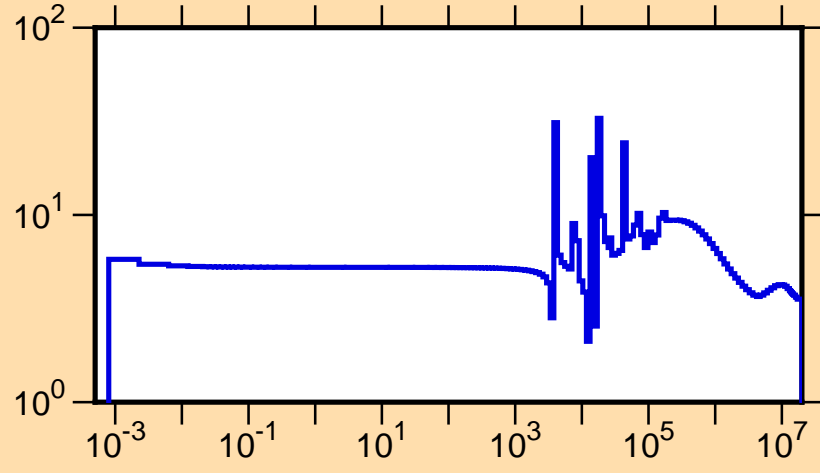
\sigma vs. E for ^{90}\text{Zr}(n,\text{tot.})
