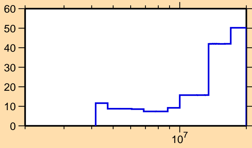
\Delta\sigma/\sigma vs. E for ^{90}\text{Zr}(n,n\text{cont.})
