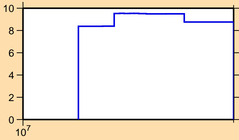
\Delta\sigma/\sigma vs. E for ^{90}\text{Zr}(n,\text{el.})
