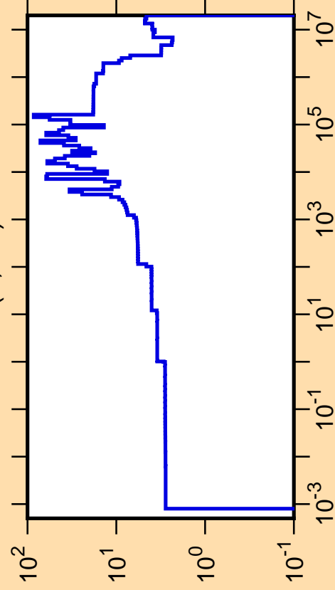
\Delta\sigma/\sigma vs. E for ^{90}\text{Zr}(n,\text{tot.})
