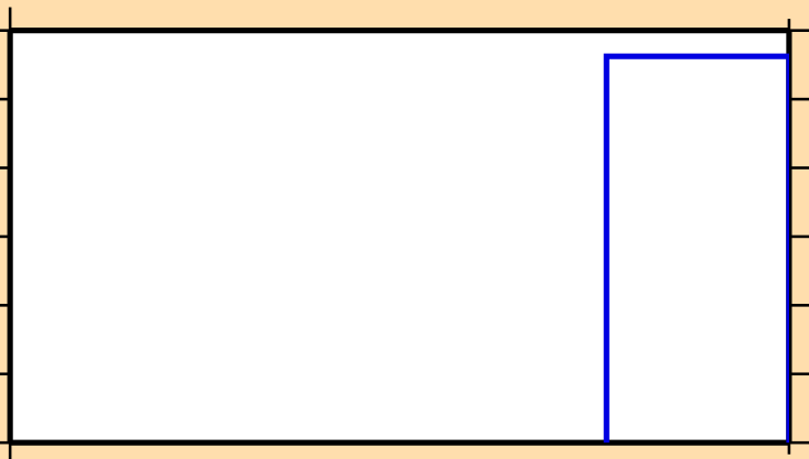
\sigma vs. E for ^{90}\text{Zr}(n,\text{nd})
