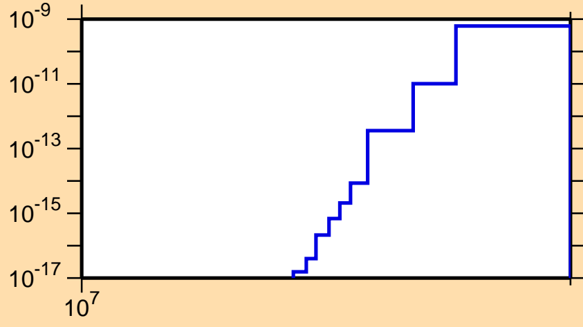
\sigma vs. E for ^{90}\text{Zr}(n,p\alpha)
