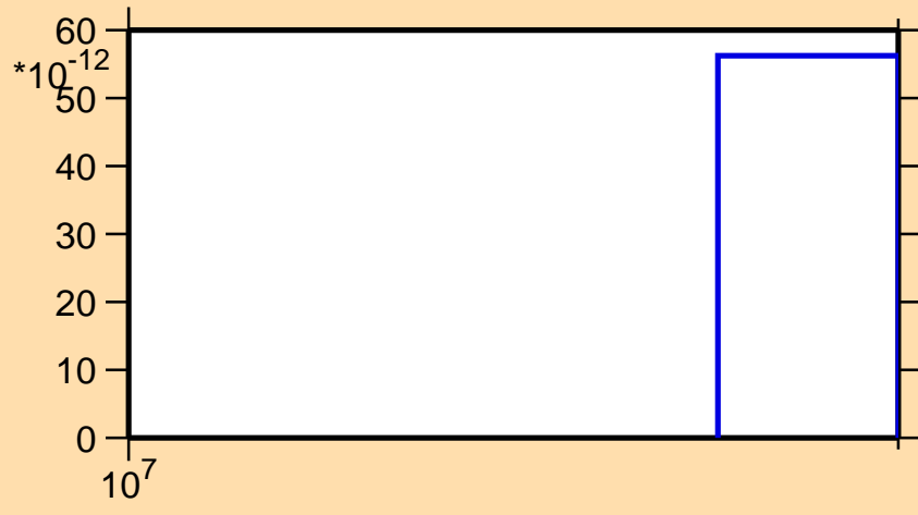
\sigma vs. E for ^{90}\text{Zr}(n,\text{nd})
