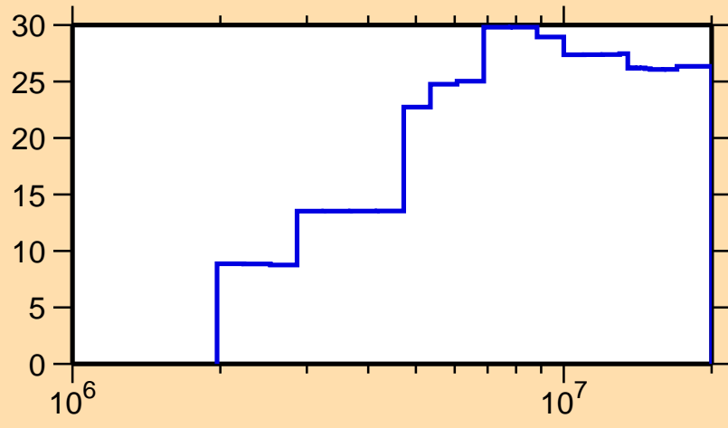
\Delta\sigma/\sigma vs. E for ^{90}\text{Zr}(n,n_1)
