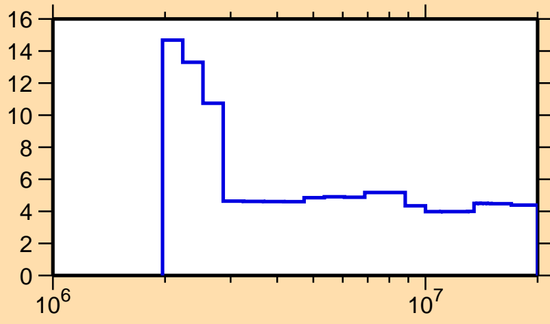
\Delta\sigma/\sigma vs. E for ^{90}\text{Zr}(n,\text{nonel.})
