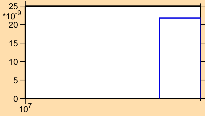
\sigma vs. E for ^{90}\text{Zr}(n,\text{pd})
