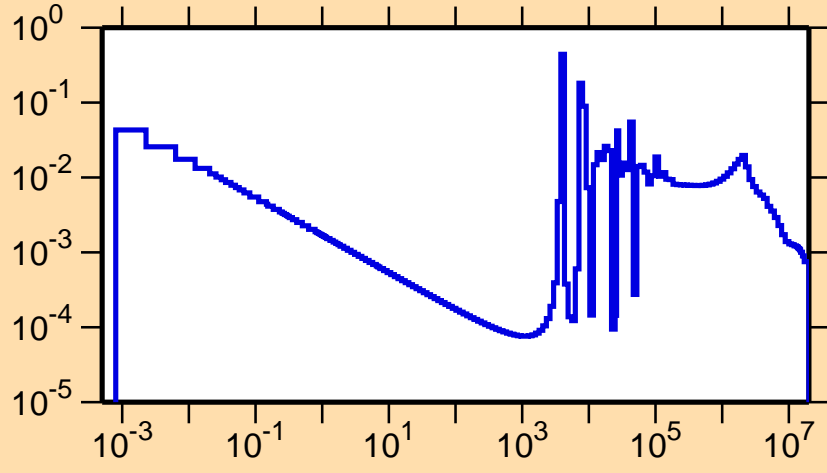
\sigma vs. E for ^{90}\text{Zr}(n,\gamma)
