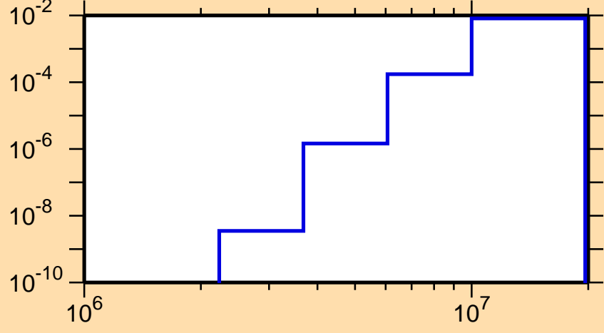
\sigma vs. E for ^{90}\text{Zr}(n,\alpha)
