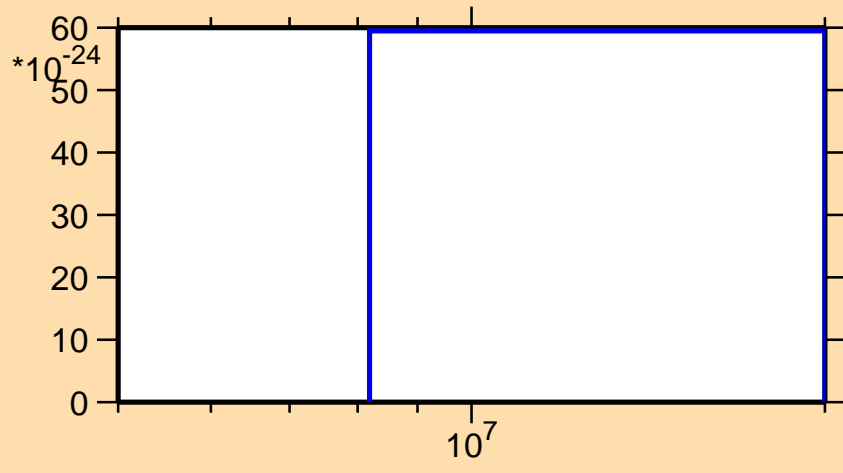
\sigma vs. E for ^{90}\text{Zr} (mt 34)
