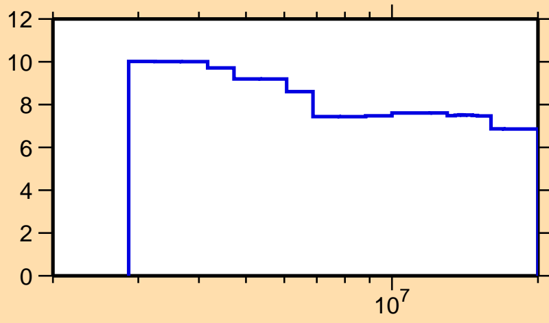
\Delta\sigma/\sigma vs. E for ^{91}\text{Zr}(n,n\text{onel.})
