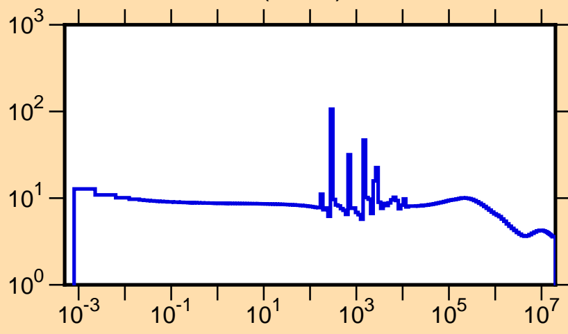
\sigma vs. E for ^{91}\text{Zr}(n,\text{tot.})
