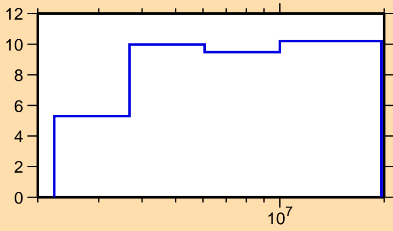
\Delta\sigma/\sigma vs. E for ^{91}\text{Zr}(n,el.)
