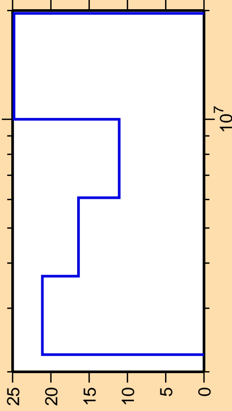
\Delta\sigma/\sigma vs. E for ^{91}\text{Zr}(n,ncont.)
