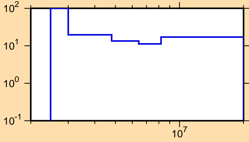
\Delta\sigma/\sigma vs. E for ^{91}\text{Zr}(n,n\text{cont.})
