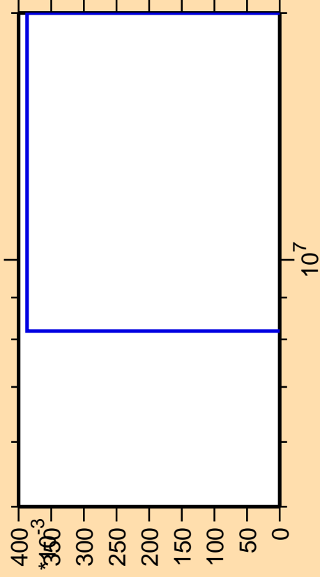
\Delta\sigma/\sigma vs. E for ^{91}\text{Zr}(n,2n\alpha)
