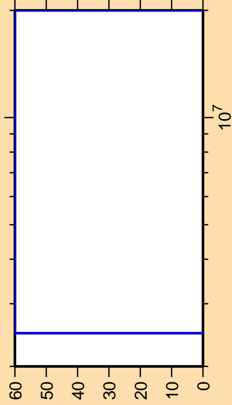
\Delta\sigma/\sigma vs. E for ^{91}\text{Zr}(n,\alpha)
