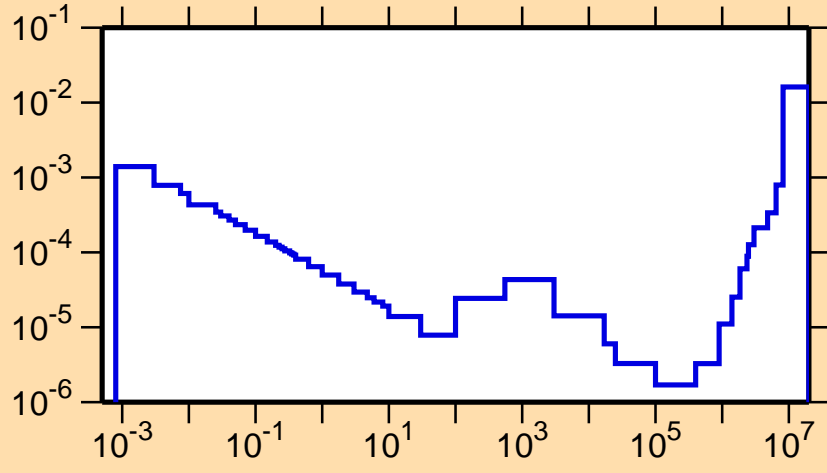
\sigma vs. E for ^{91}\text{Zr}(n,\alpha)
