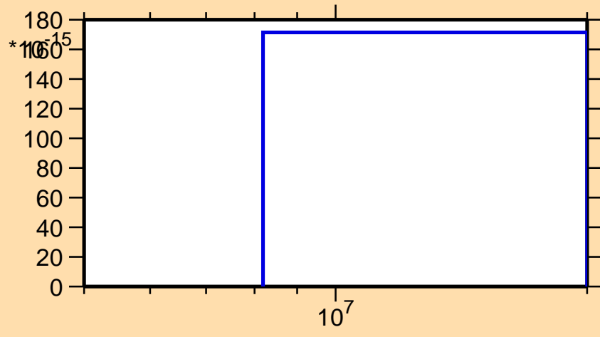
\sigma vs. E for ^{91}\text{Zr}(n,2n\alpha)
