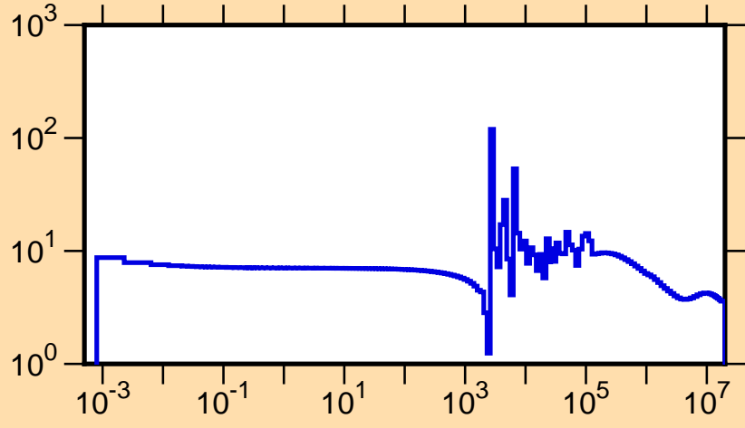
\sigma vs. E for ^{92}\text{Zr}(n,\text{tot.})
