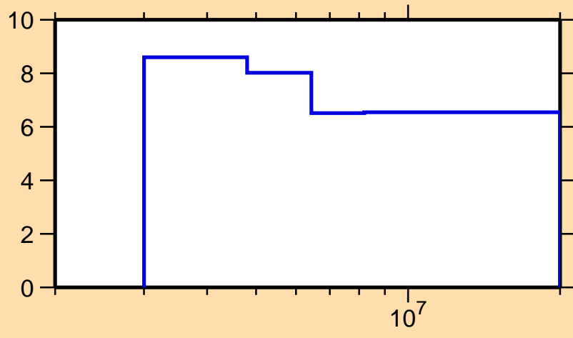
\Delta\sigma/\sigma vs. E for ^{92}\text{Zr}(n,n\text{onel.})
