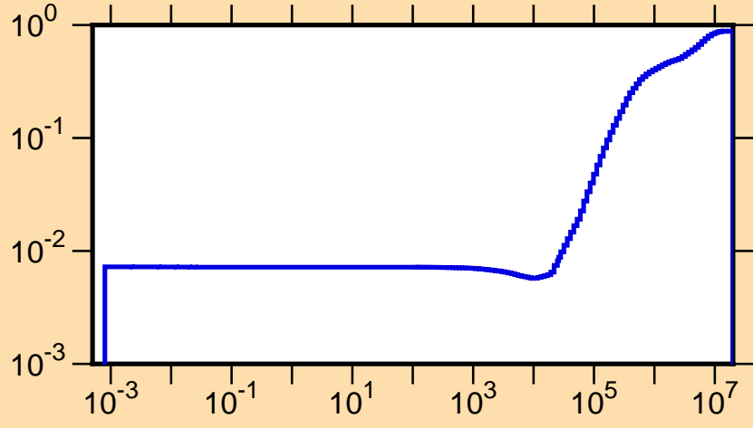
\mu vs. E for ^{93}\text{Zr}(\text{mt251})
