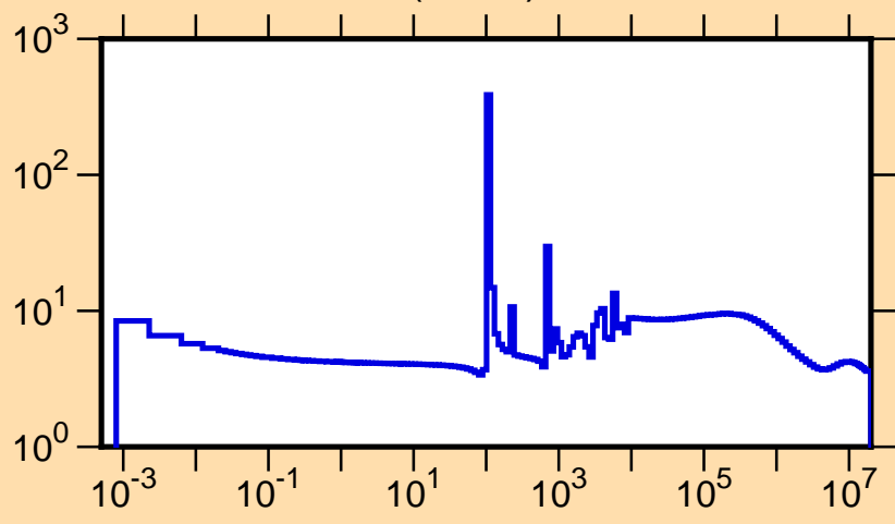
\sigma vs. E for ^{93}\text{Zr}(n,\text{tot.})
