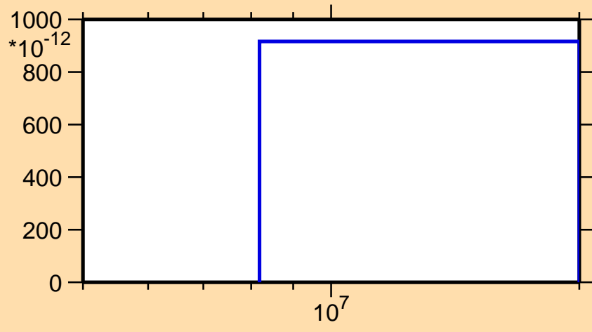
\sigma vs. E for ^{93}\text{Zr}(n,2np)
