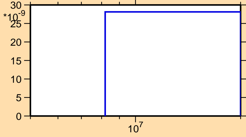
\sigma vs. E for ^{93}\text{Zr}(n,\text{nd})
