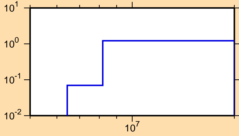
\sigma vs. E for ^{93}\text{Zr}(n,2n)
