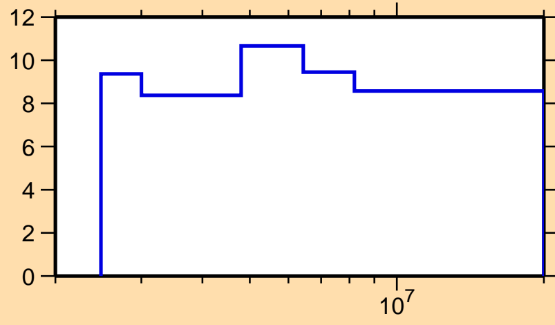
\Delta\sigma/\sigma vs. E for ^{93}\text{Zr}(n,n\text{onel.})
